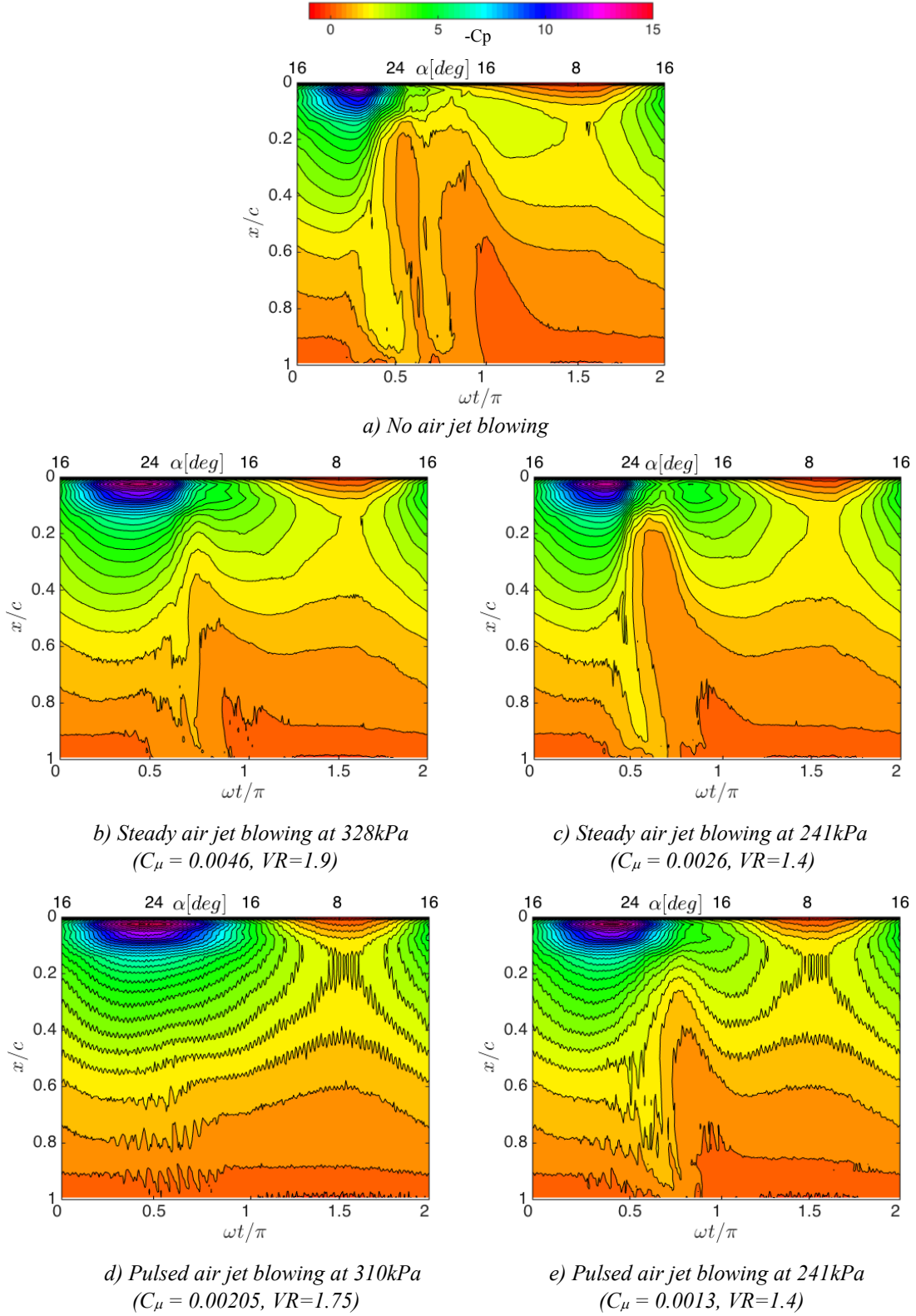
Fig 8. Comparison between upper surface pressure distribution versus \alpha for steady and pulsed ( f=71\text{Hz} , F^+=1.04 ) air jet blowing at \sim 310\text{kPa} and \sim 241\text{kPa} , \bar{\alpha}=16^\circ , \hat{\alpha}=\pm 8^\circ , \omega=12.38\text{rad/s} ( k=0.103 ) pitching, U_\infty=30\text{m/s} , Re_c=1.0\times 10^6
