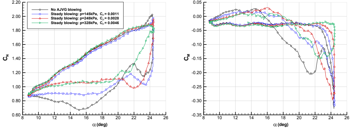
a) Steady air jet blowing
