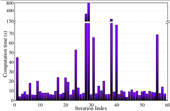
Fig. 5 The CPU time of (35)-(36) for a scenario in the 30-scenario case
