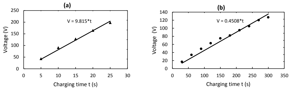
Fig. 6. (a) test result for configuration B (30nF); (b) test result for configuration B (1 \mu F).
