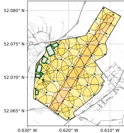
Fig. 4. The patrolling waypoints generated in Cranfield Airport scenario. Grid size in discretization is 100 meters, and the visibility range of drones is assumed to be 300 meters
