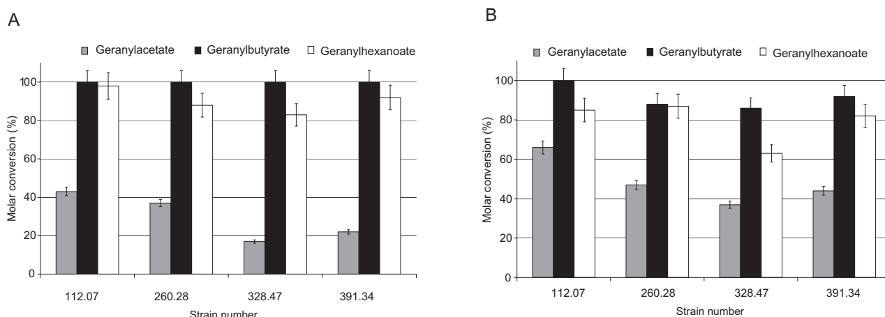
FIG. 3 - Formation of geranyl esters catalysed by Rhizopus oryzae strains grown on solid-state media (A) and in submerged cultures (B). Molar conversions refer to 24 h of reaction.
