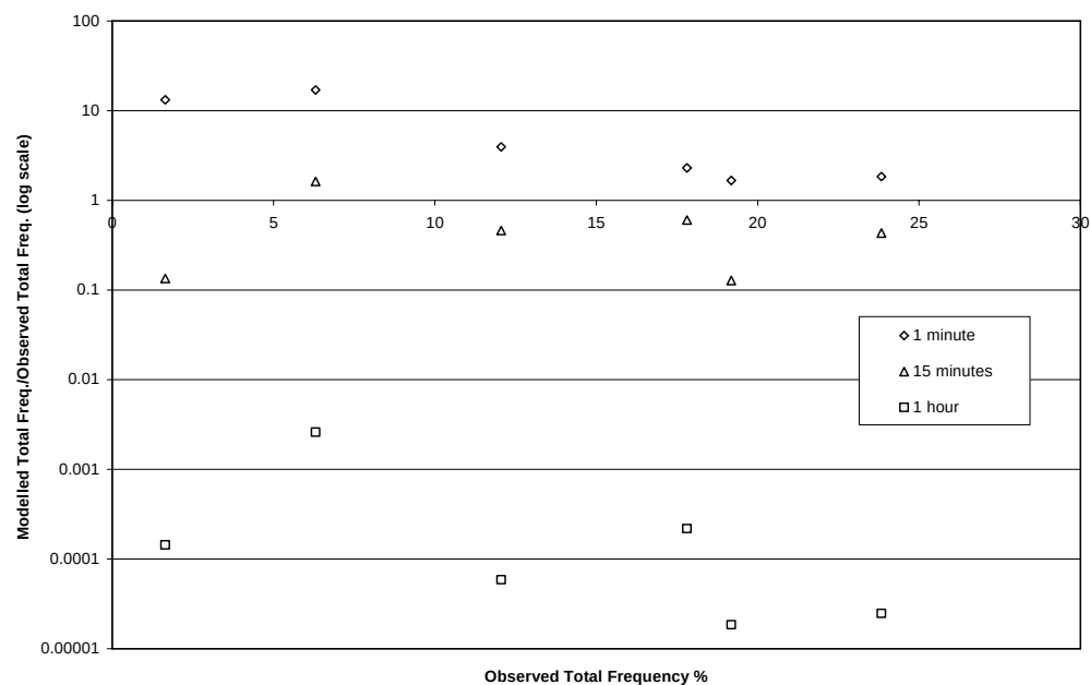
Fig. 6 The ratio of modelled to observed frequencies for an odour concentration of 2 \text{ ou}_E/\text{m}^3 .
