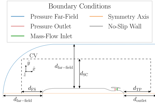
Fig. 7. Schematic of the domain, propulsive fuselage model, boundary conditions and analysis control volume.
