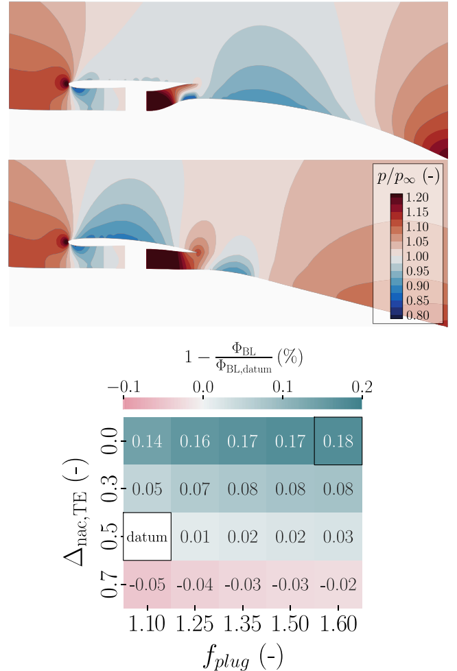
Fig. 15. Normal static pressure contours from the two boxed designs (datum on bottom) with the computed difference in viscous dissipation rate within the BL between datum and the geometries at BLR = 50% and FPR = 1.30.
