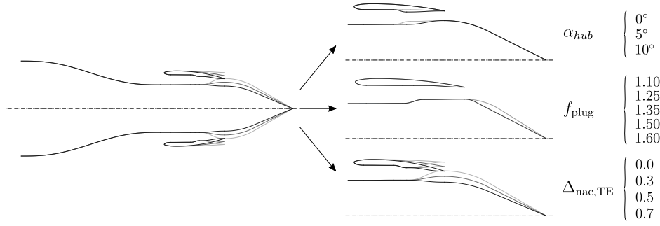
Fig. 8. Variations in the exhaust and plug design, following the design variables defined in Fig. 5.
