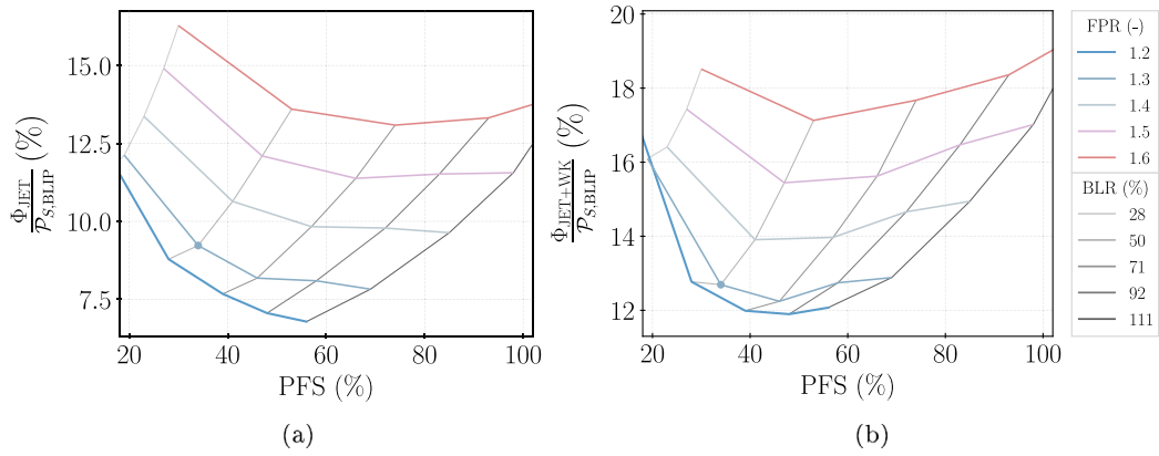
Fig. 20. Computed portion of viscous dissipation rate in (a) the jet and (b) the jet and wake, relative to the power demand from the aft-mounted fan to provide the pressure rise targeted.
