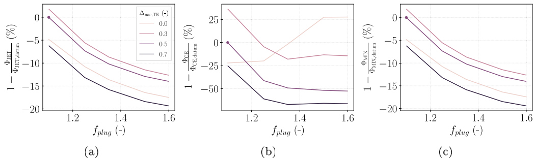
Fig. 17. Computed relative difference in viscous dissipation rate in the (a) jet plume, (b) core-expansion, and (c) jet/wake mixing at BLR = 50% and FPR = 1.30 with datum (marker).
