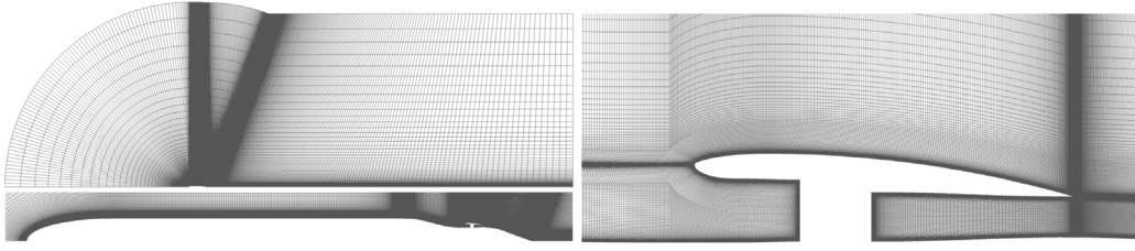
Fig. 6. Coupled C-structure grid around a propulsive fuselage with the mesh of the domain, around the fuselage and around the propulsor.
