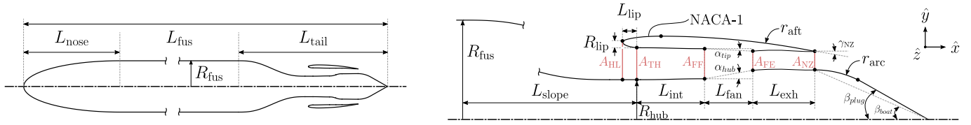
Fig. 5. Schematic of an axi-symmetric fuselage with a thruster, with its tail slope, propulsor intake, cowl, exhaust, and aft-cone geometries parametrisation (black) and thermodynamic stations (pink). (For interpretation of the references to colour in this figure legend, the reader is referred to the web version of this article.)
