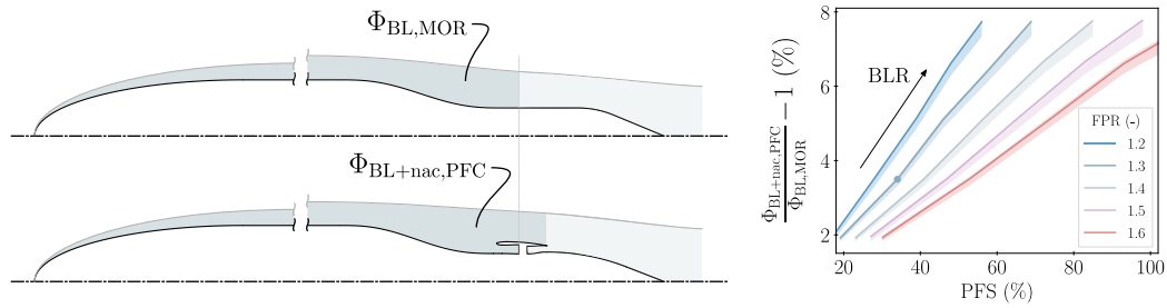
Fig. 13. Integration penalties in terms of viscous dissipation rate between the installed nacelle configuration (PFC) and the baseline morphed fuselage (MOR) with respect to different propulsor sizes, fan operating conditions (colours) and nacelle shapes as explored (shaded areas), with an identified datum (marker) for further comparisons.
