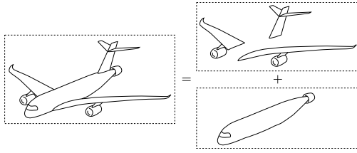
Fig. 2. Decomposition of the propulsive fuselage concept into partial assemblies: fus+P at bottom and rest at top.
