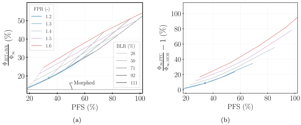
Fig. 21. Computed (a) portion of viscous dissipation rate in the jet and wake relative to the wake of the baseline morphed fuselage (MOR) with respect to different propulsor sizes, fan operating conditions and (b) total viscous losses between the powered and unpowered fuselages.
