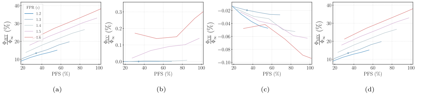
Fig. 16. Computed portion of the viscous dissipation rate in the (a) jet plume, (b) core-compression, (c) core-expansion, and (d) jet/wake mixing regions relative to the overall viscous loss with the previously identified datum design (marker).
