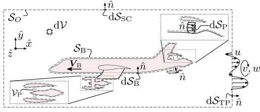
Fig. 1. Schematic of a control volume encapsulating a powered aerodynamic body.
