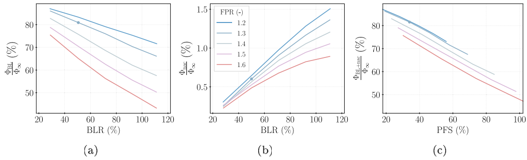
Fig. 14. Computed non-dimensional dissipation in the (a) main, (b) secondary and (c) combined boundary layers for different BLR and FPR combinations, and datum (marker).
