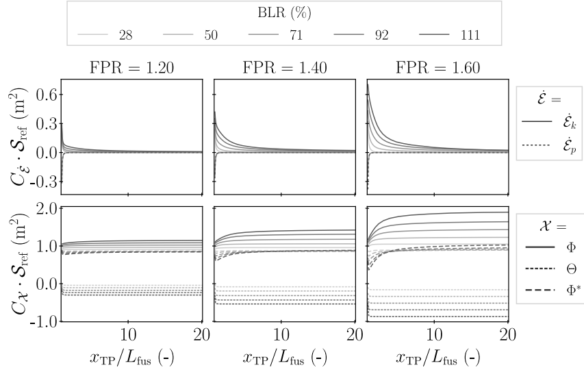
Fig. 9. Computed energy flux transfer between the kinetic energy deposition rate and the volumetric rate of viscous dissipation, pressure work and overall sink for various BLR and FPR.
