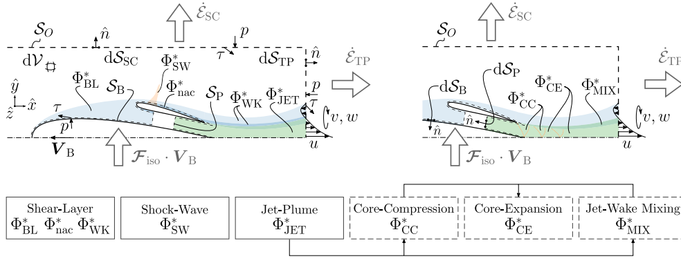
Fig. 3. Flow-chart of the precedence process for work flow-paths identification and schematic of the corresponding mechanisms.
