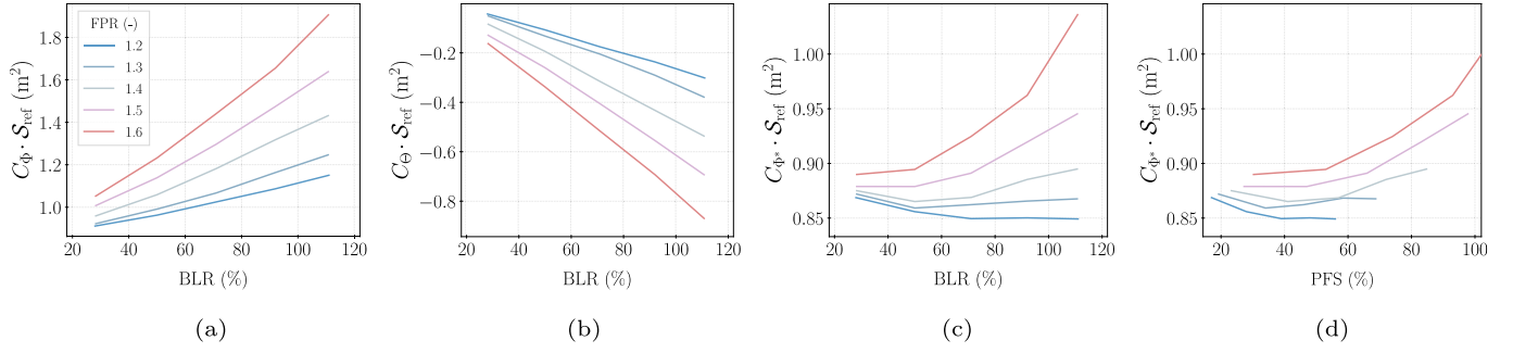
Fig. 10. Computed volumetric rate of (a) viscous dissipation, (b) pressure work, and overall losses as a function of (c) BLR and (d) PFS.
