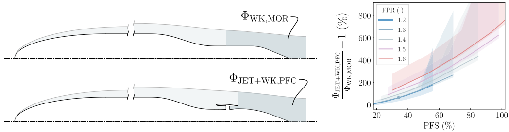
Fig. 19. Viscous dissipation rate attenuation within the jet and wake between the installed nacelle configuration (PFC) and the baseline morphed fuselage (MOR) with respect to different propulsor sizes, fan operating conditions and nacelle shapes as explored (shaded areas), with the previously identified datum design (marker).
