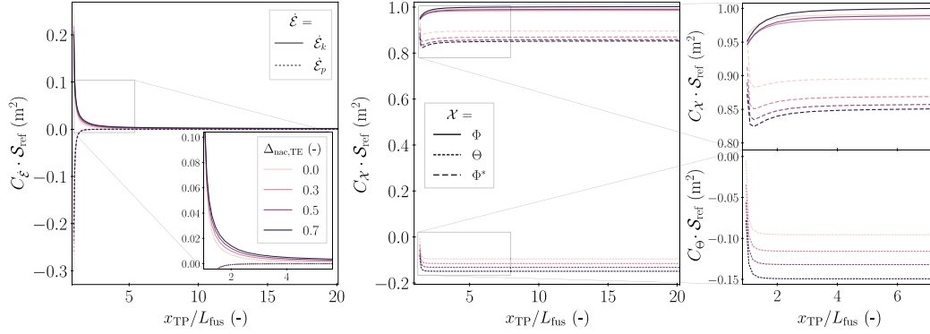
Fig. 11. Computed energy flux transfer between the kinetic energy deposition rate and the volumetric rate of viscous dissipation, pressure work and overall sink as a function of the nacelle droop.
