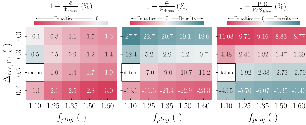
Fig. 12. Computed volumetric rate of viscous dissipation and pressure work, and propulsive force share as a function of droop and plug angles, at datum BLR = 50% and FPR = 1.30, neglecting hade angle effects.
