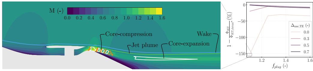
Fig. 18. Mach number contours of the boxed geometry at BLR = 92%, FPR = 1.50, \alpha_{hub} = 0^\circ , f_{plug} = 1.10 and \Delta_{nac,TE} = 0.0 , and droop and plug angles effects on the jet viscous dissipation rate.
