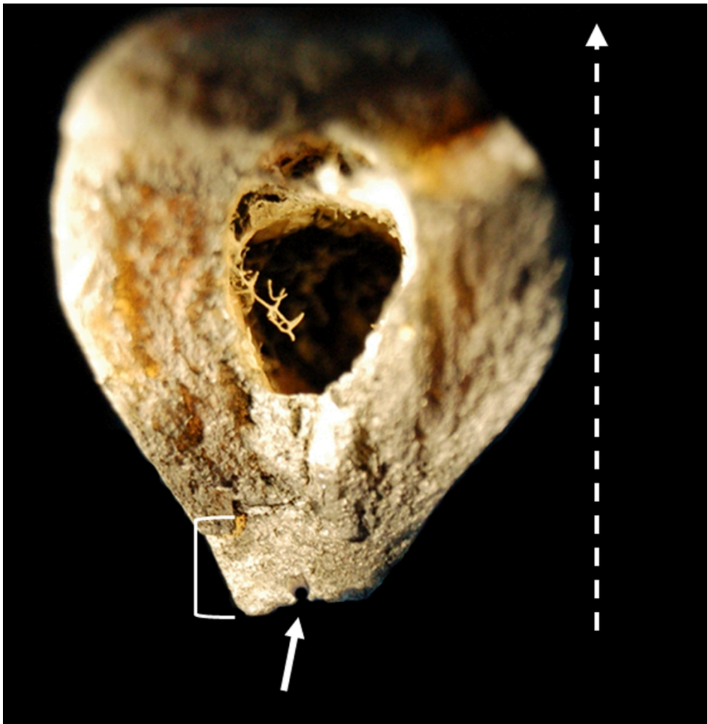
Figure 3: Crack origin at the site of a nutrient foramen opening; solid arrow indicates the nutrient foramen opening on a posterior human femur, bracket indicates the mirror zone, and the dashed arrow indicates the direction of crack propagation.
