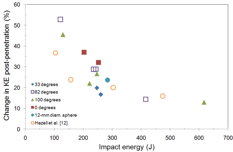
Fig. 4. Variation of change in kinetic energy post-impact (%) with initial projectile impact energy for the varying projectiles considered here, plus data from Ref. [12].
