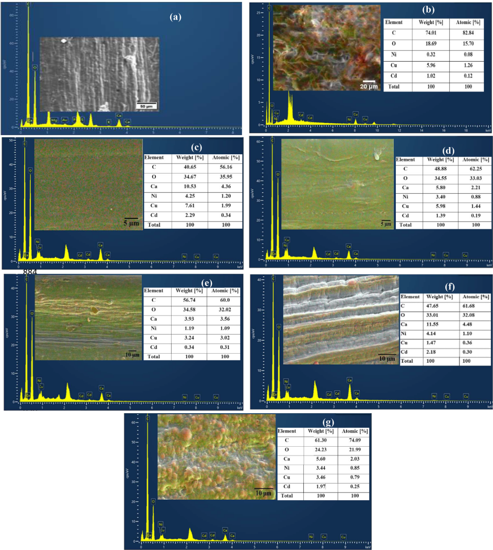
Fig. 9. Detailed SEM-EDX morphology and elemental peaks of composites: (a) Pure SAlg-MoF (0.4 %), (b) Absorbed MoP (b), (c) SAlgF, and SAlg-MoF (d) 0.5 %, (e) 1 %, (f) 4 %, and (g) 8 %, after selective adoption of heavy ions ( \text{Cu}^{2+} , \text{Ni}^{2+} , and \text{Cd}^{2+} ).
