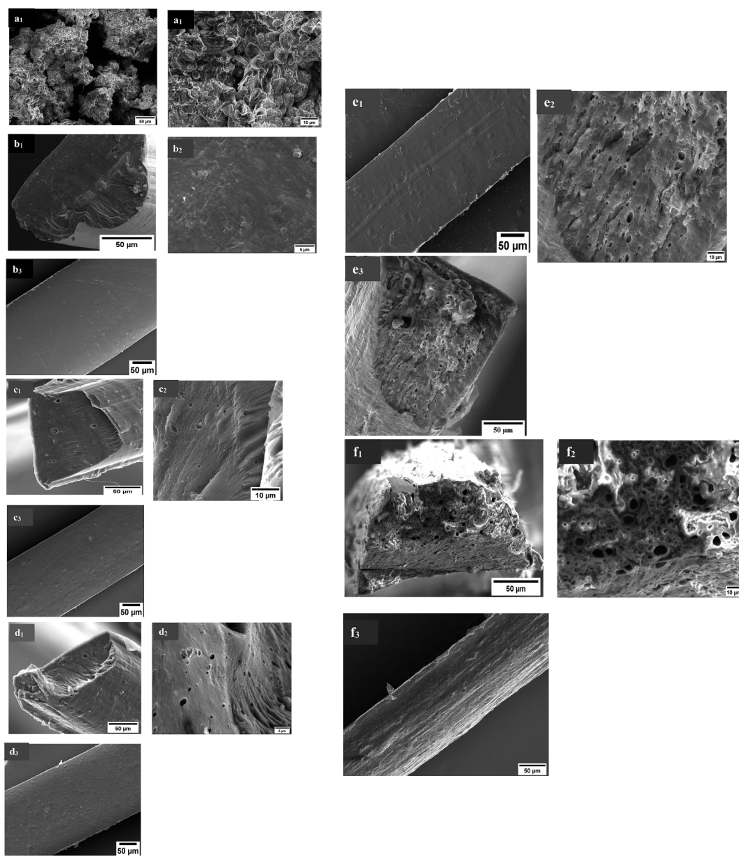
Fig. 5. Scanning electron microscopy (SEM) images displaying morphological details of materials at different magnifications. MoP (a 1 : 800x, a 2 : 3000x), SAlgF cross-sections (b 1 : 800x, b 2 : 3000x) and surface (b 3 : 800x), along with SAlg-MoF composites (0.5 %–8 % MoP; c 1 –f 3 ) at 800x and 3000x magnifications to show morphological variations.
