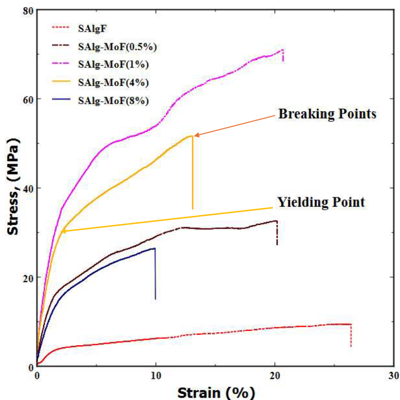
Fig. 6. The stress-strain curves of the SAlgF and SAlg-MoF composites.
