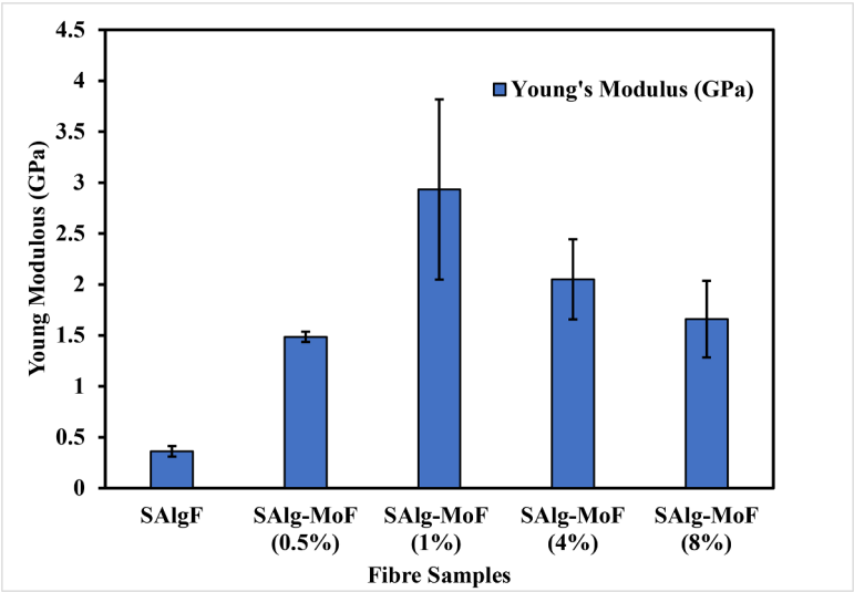
Fig. 8. Typical Young modulus of SAlgF and SAlg-MoF Composites.
