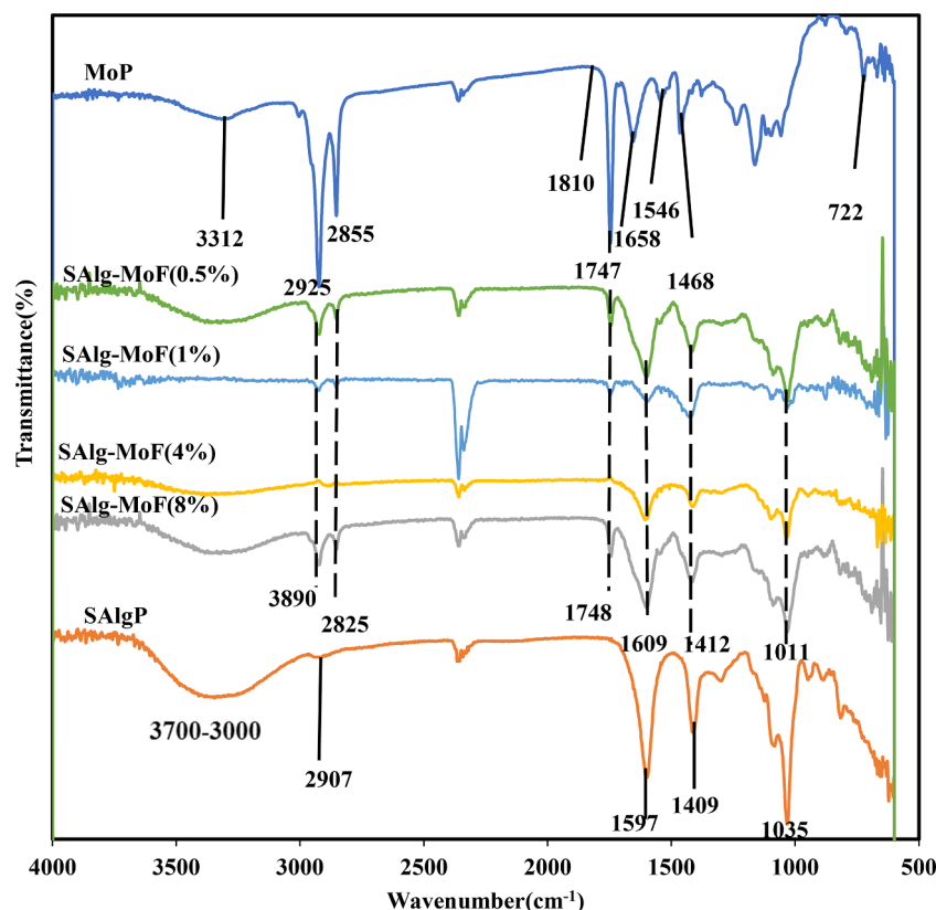
Fig. 2. FTIR spectra comparing the transmittance of MoP, SAlgP, and SAlg-MoF (0.5 %–8 %), composites at varying concentrations.
