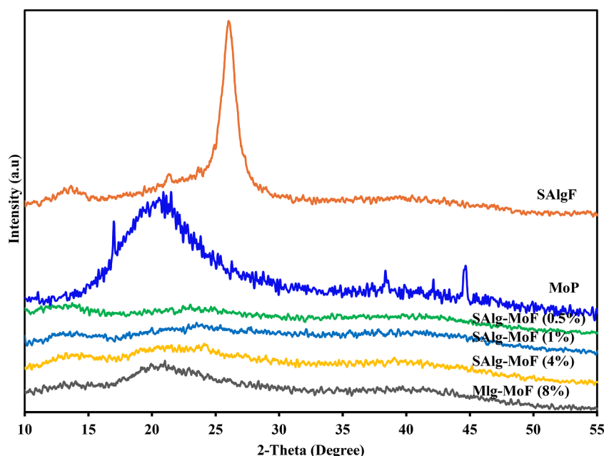
Fig. 4. X-ray diffraction (XRD) patterns analysis of MoP, SAlgF, and SAlg-MoF composites (0.5 %, 1 %, 4 %, and 8 % MoP) indicating phase composition.
