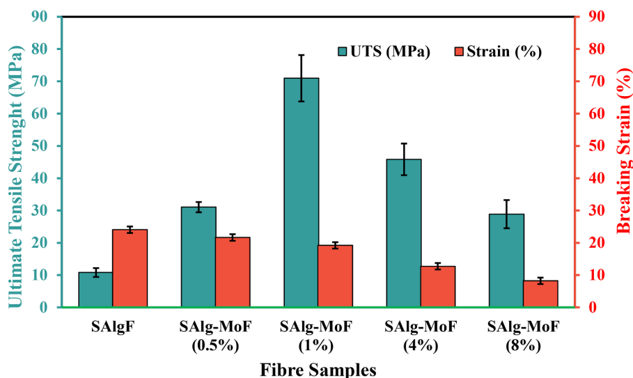
Fig. 7. Combination plot of the ultimate tensile strength and breaking strain of SAlgF and SAlg-MoF Composites.
