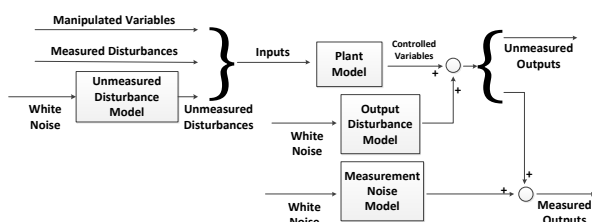
Figure 12: Model Predictive Control Algorithm – MATLAB toolbox [13]
