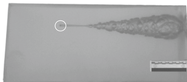
Fig. 4 Example of a 5.5 mm diameter steel ball bearing (impact velocity = 654 m/s) penetrating a 250 mm × 250 mm × 500 mm gelatine block (10% by mass, conditioned to 4 °C). Maximum temporary cavity is shown and the final position of the ball bearing is circled.
