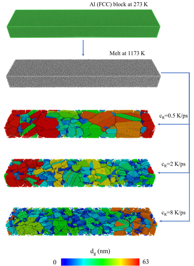
Fig. 1. Workpiece grain structures following cooling and equilibration.
