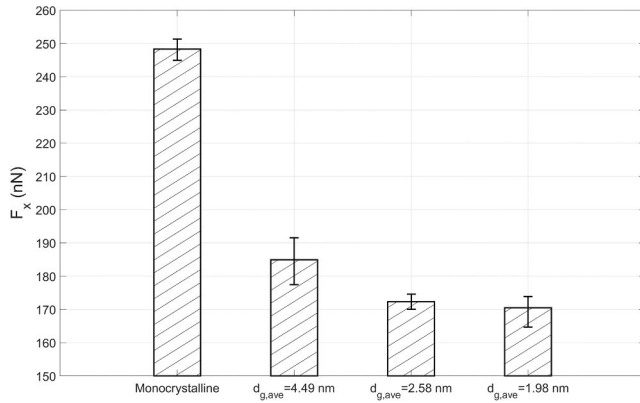
Fig. 8. Average tangential forces ( F_x ) vs. grain structure.
