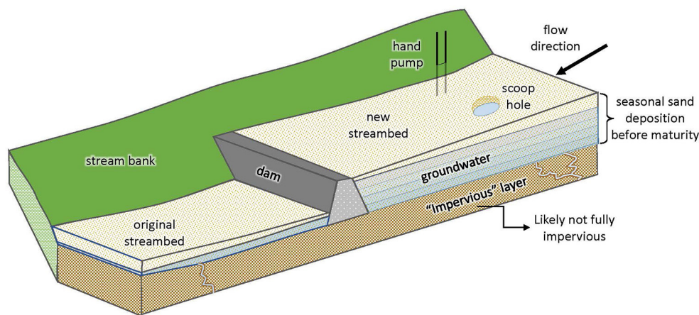
FIGURE 2 | Sand dam schematic showing seasonal sand deposition before maturity and two common abstraction methods (adapted from Eisma and Merwade, 2020).
