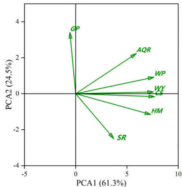
Fig. 3. Biplot of ecosystem services for the first two PCA axes (85.8% of the variability absorbed. ES indicators are: GP-grain production; WY-water yield; WP-water purification; SR-soil retention; CS-carbon storage; AQR-air quality regulation; and HM-habitat maintenance).
