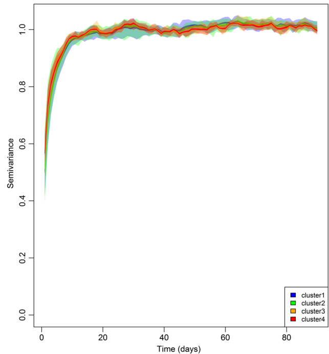
Figure 5. Semi-variograms from daily precipitation data for the four identified clusters with the mean of each cluster (line) and the 95% confidence intervals (shaded area)
