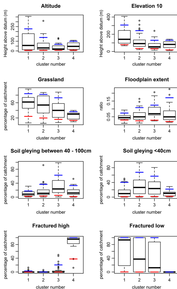
Figure 7. Box plots of characteristics which differ between two or three clusters, as in Figure 6
