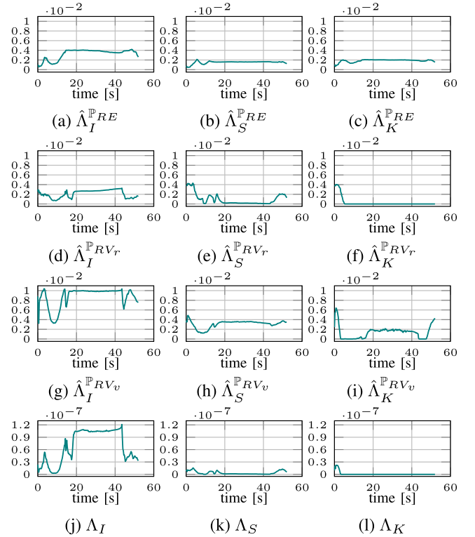
FIGURE 10 (a)–(i) Interpolated trajectory likelihood of image acquisition scenario corresponding to each phase plane. The final computed intention likelihood of image acquisition, smuggling, and kamikaze are shown in (j), (k), and (l), respectively.
