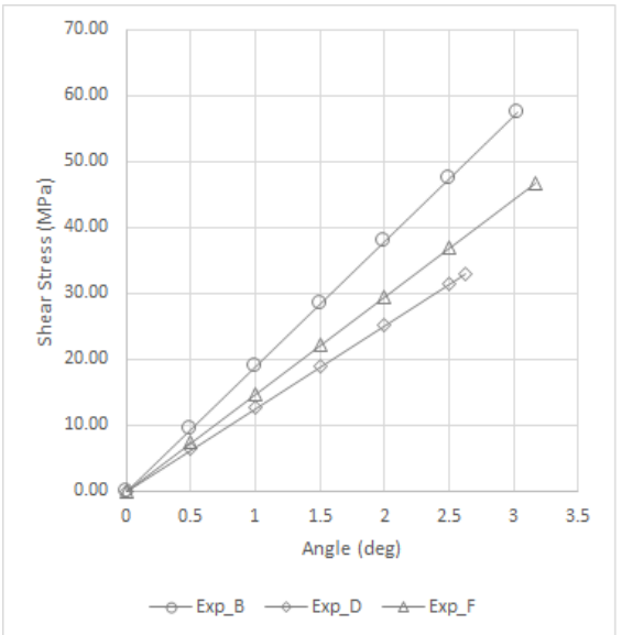
Figure 16: Shear Stress vs Angle of twist (High Temperature Cured)
