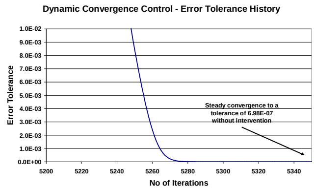
Fig. 11 Typical convergence history using Newton's method with no DCC algorithm intervention
