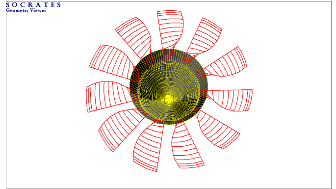
Fig. 6 Example of SOCRATES ' turbomachinery design environment – single stage fan with cone
