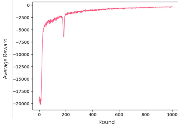
Fig. 5. Average reward during training.
