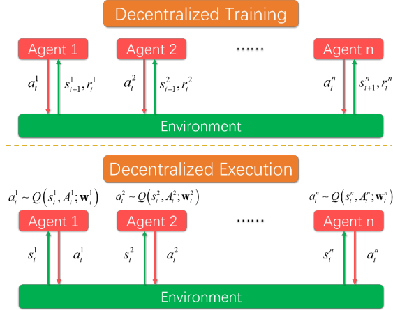
Fig. 3. Schematic diagram of decentralized training with decentralized execution.
