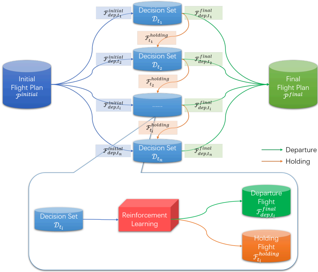
Fig. 1. DCB sequence decision framework based on time window.
