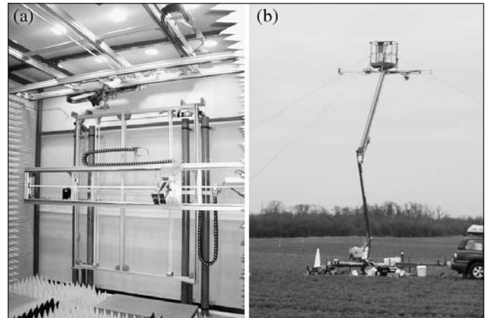
Figure 1. (a) View looking to one end of the anechoic chamber showing the 2.5 m × 3.7 m roof-mounted and 1.9 m × 3.7 m wall-mounted 2D scanners. The polarimetric antenna cluster is visible, as are the coaxial chain-link feeds. (b) The outdoor system deployed for imaging which scans the antenna head along a 4 m horizontal linear scanner.
