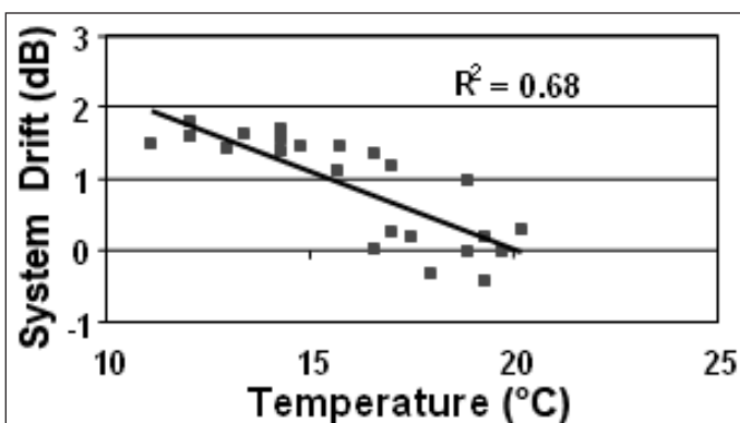
Figure 8. Correlation between the system drift, as measured by the coupled signal, and temperature recorded by the weather station at the top of the hoist.
