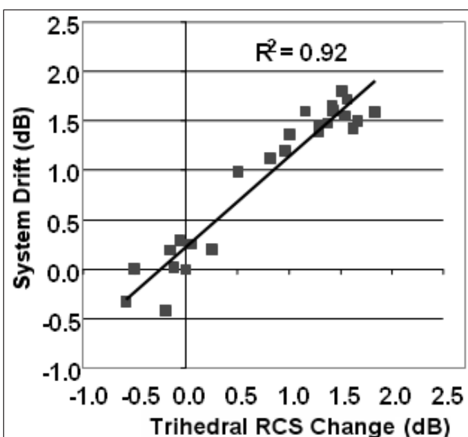
Figure 9. Correlation between the HH system drift as measured by the coupled signal and that measured by the variation in the RCS of a trihedral extracted from the sequence of SAR images.
