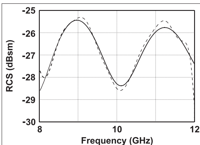
Figure 3. Comparison of the measured X-band response (broken line) and theoretical prediction (solid line) for the 6.4 cm sphere used in the indoor system calibration procedure. The apparent discrepancies at the edges of the frequency range are due to data windowing.
