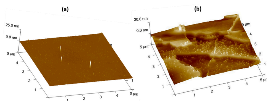
Figure 4. Bare Si wafer (a) and PEGylated IONPs dried on Si wafer (b).
