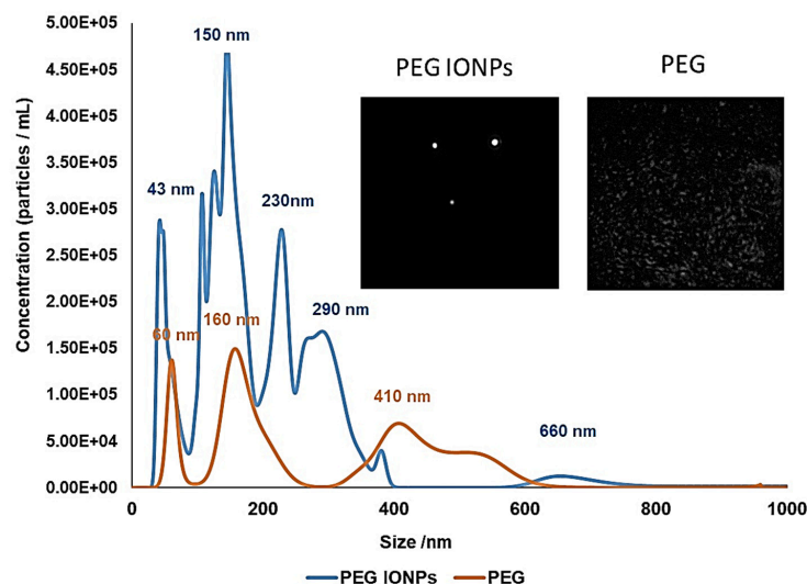
Figure 6. NTA measurements of concentrated PEG IONPs solution (blue) and concentrated PEG solution (orange), as control. Histograms are average of 3 measurements. Insets show screenshots of representative NTA video for both PEG IONPs and PEG only solutions.
