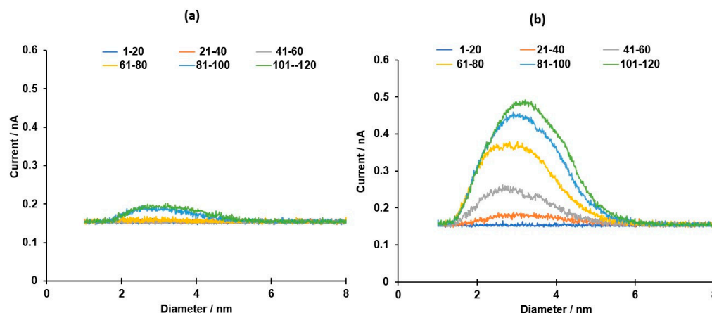
Figure 1. Low (a) and high (b) power spectra of \text{Fe}_3\text{O}_4 .
