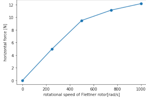
(a) The relationship between the Magnus force and Flettner rotor speed
