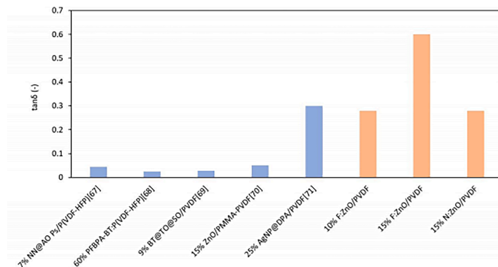
Fig. 12. Summary of tan \delta of polymer-based nanocomposites at 1 kHz and comparison with literature data.
