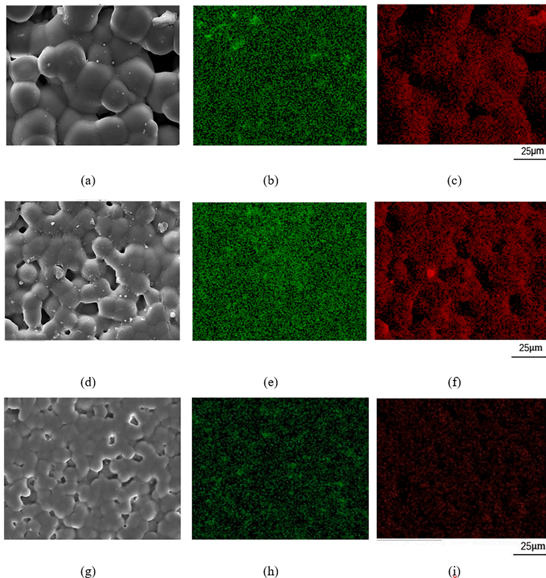
Fig. 7. (a) SEM image of PVDF + 15 wt% ZnO; (b) Zn distribution of PVDF + 15 wt% ZnO; (c) O distribution of PVDF + 15 wt% ZnO; (d) SEM image of PVDF + 15 wt% F:ZnO; (e) Zn distribution of PVDF + 15 wt% F:ZnO; (f) O distribution of PVDF + 15 wt% F:ZnO; (g) SEM image of PVDF + 15 wt% N:ZnO; (h) Zn distribution of PVDF + 15 wt% N:ZnO; and (i) O distribution of PVDF + 15 wt% N:ZnO.
