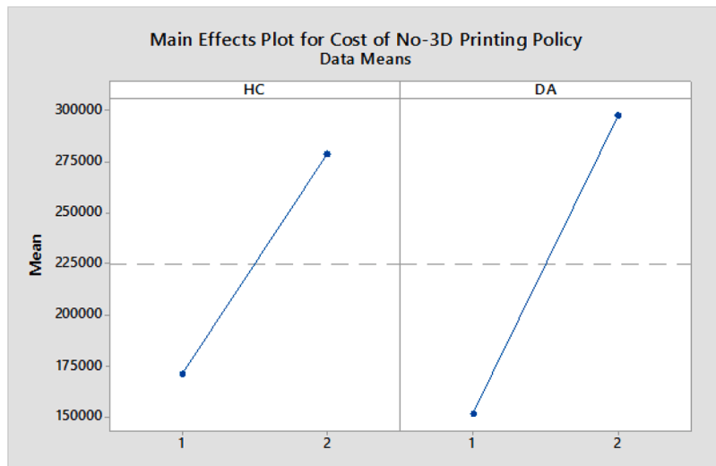
Fig. 12b. Main effects plot for no-3D printing policy.
