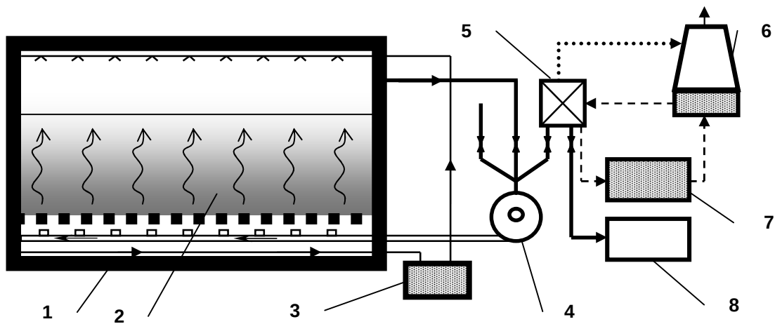
Fig. 1. Schematic of biodrying box with process air circulation and dehydration based on a Herhof system: (1) enclosed box; (2) air forced through the waste matrix, heated by the exothermic aerobic biodegradation of readily decomposable waste fragments; (3) leachate collection and circulation system; (4) forced aeration system with partial air re-circulation, mixing ambient air and conditioned process air; (5) heat exchanger; (6) cooling tower; (7) water (vapour condensate); (8) exhaust air treatment through biofilter or regenerative thermal oxidation (RTO). Appropriate conditions for microbial activity allow for the biodegradation of the waste placed within the bioreactor, providing the necessary heat to evaporate moisture from the waste fragments. Evaporated moisture is removed by the air convection, achieved by forced aeration. The exhaust air is going through various treatment stages that improve its drying capacity (ability to carry moisture) before it is partly re-circulated into the reactor, after being mixed with ambient air. Redrawn from Herhof Environmental (Undated).
