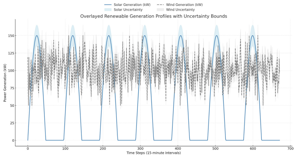
Fig. 2. Overlaid renewable generation profiles with uncertainty bounds.
