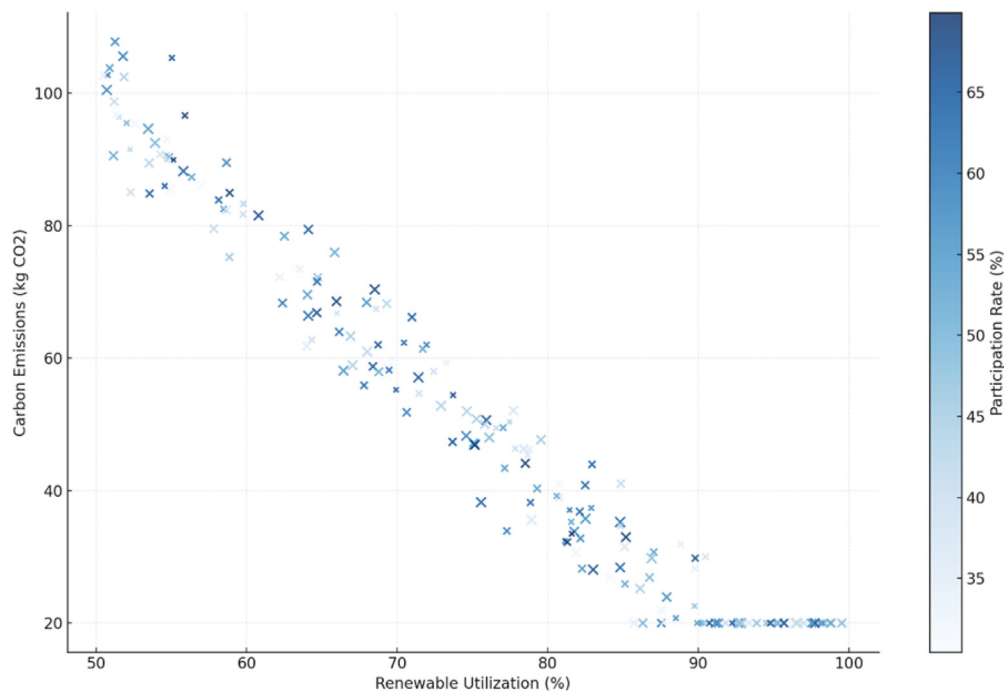
Fig. 6. Scatter plot of renewable utilization vs. Carbon emissions.
