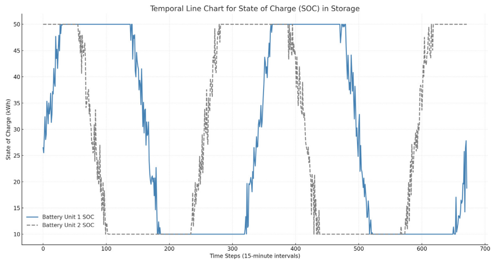
Fig. 4. Temporal line chart for state of charge in storage.
