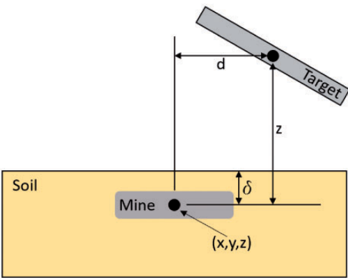
Figure 2. ‘Initial Impulse Mine’ model where the explosive charge was modelled as point of charge relative to the depth of burial, standoff distance, and soil density; adapted from [54].
