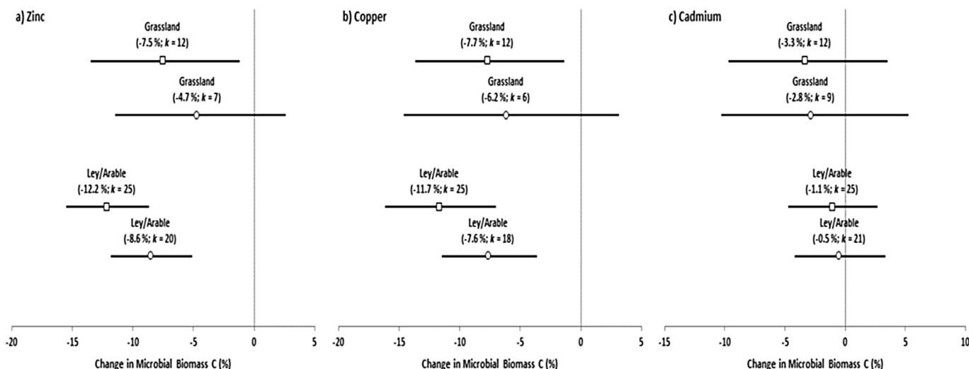
Fig. 2. Forest plots showing effects of the a) Zn, b) Cu, and c) Cd sludge treatments on microbial biomass carbon (%) grouped according to the land management practices implemented at each field site. Each point represents the summary effect sizes determined by including (□) and excluding (○) data for soils where the mean total metal concentration during the LTSE exceeds the respective UK statutory limit. The number of primary studies ( k ) used to calculate each effect size is indicated. Horizontal lines represent 95% confidence limits. Effects are not statistically significant if 95% confidence limit crosses the zero line.
