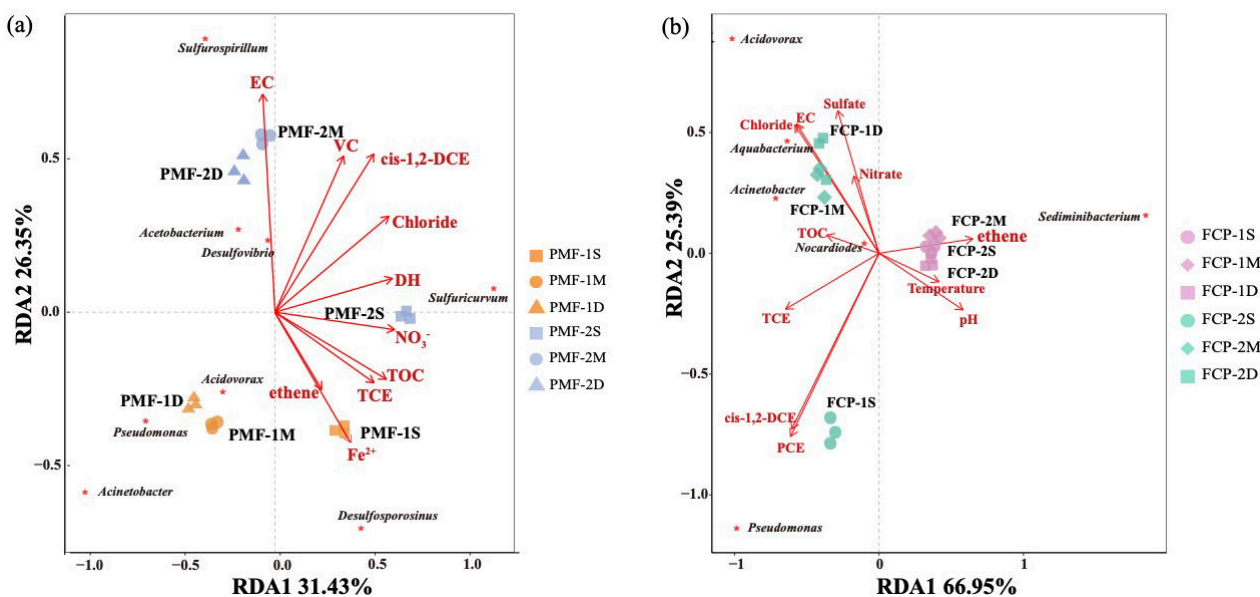
Fig. 6. Key environmental factors shaping the CE-degrading bacteria compositions in groundwater microbial community at the PMF (a) and FCP (b) site.
