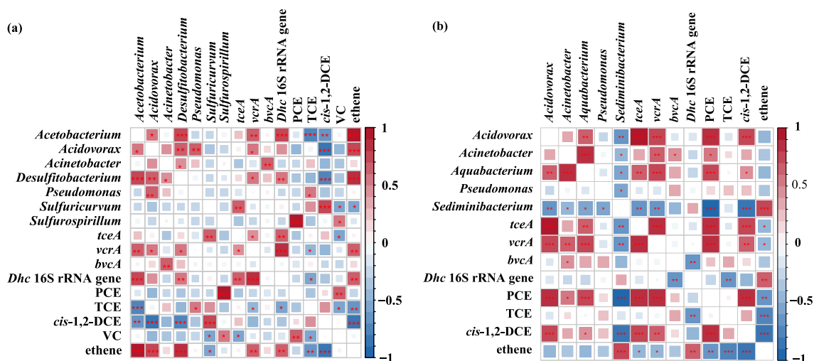
Fig. 7. Relationships between degrading bacteria, Dhc 16S rRNA, and RDase genes and CEs with ethene in groundwater at sites PMF (a) and FCP (b). *** p \leq 0.001 ; ** 0.001 < p \leq 0.01 ; * 0.01 < p \leq 0.05 .
