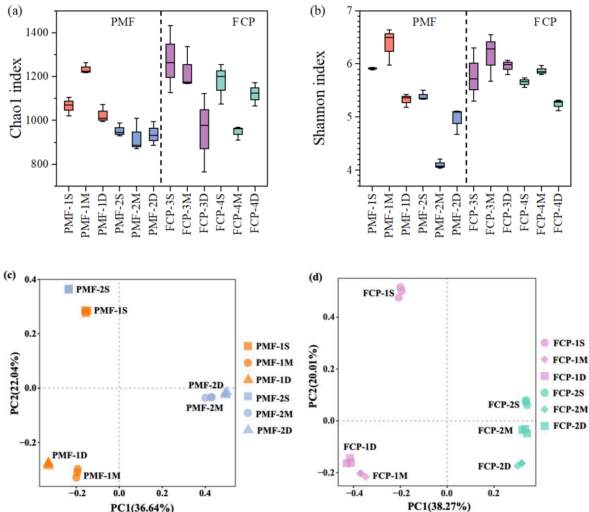
Fig. 3. Alpha diversity indices Chao1 index (a) and Shannon index (b) of the bacterial community and principal coordinates analysis based on weighted UniFrac scores on ASVs level of groundwater samples collected at sites PMF (c) and FCP (d).
