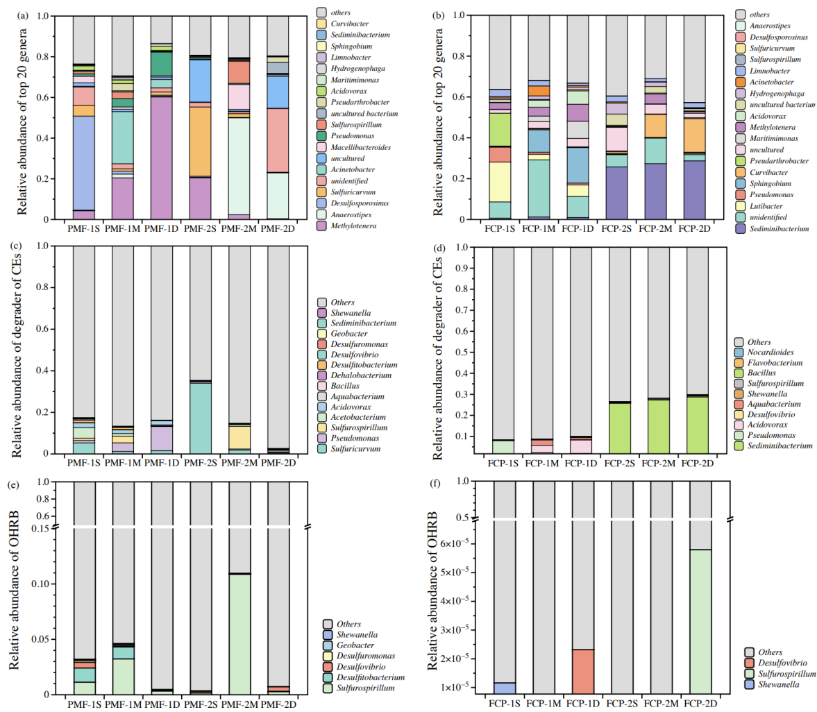
Fig. 4. Relative abundance of top 20 genera in the microbial consortium, degraders of CEs, and OHRB in groundwater at sites PMF (a, c, e) and FCP (b, d, f).
