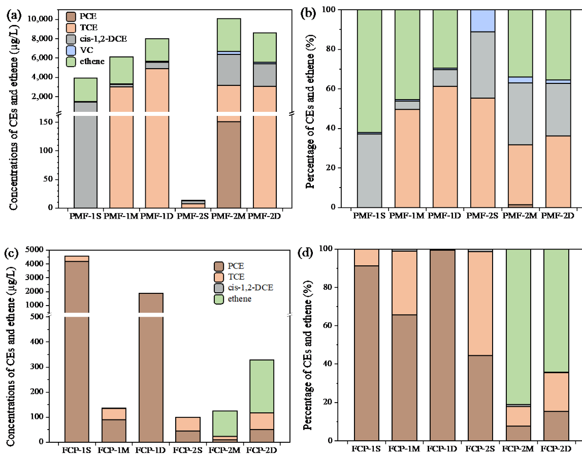
Fig. 2. Concentration and percentage of CEs and ethene in groundwater collected at the PMF (a, b) and FCP (c, d) sites.
