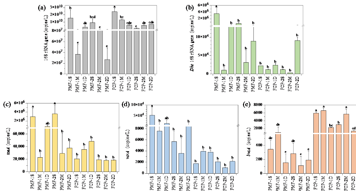
Fig. 5. Abundance of 16S rRNA gene (a), Dhc 16S rRNA gene (b), tceA (c), vcrA (d) and bvca (e) in groundwater collected at the PMF and FCP sites. Different letters showed significant differences ( p \leq 0.05 ) among the samples.
