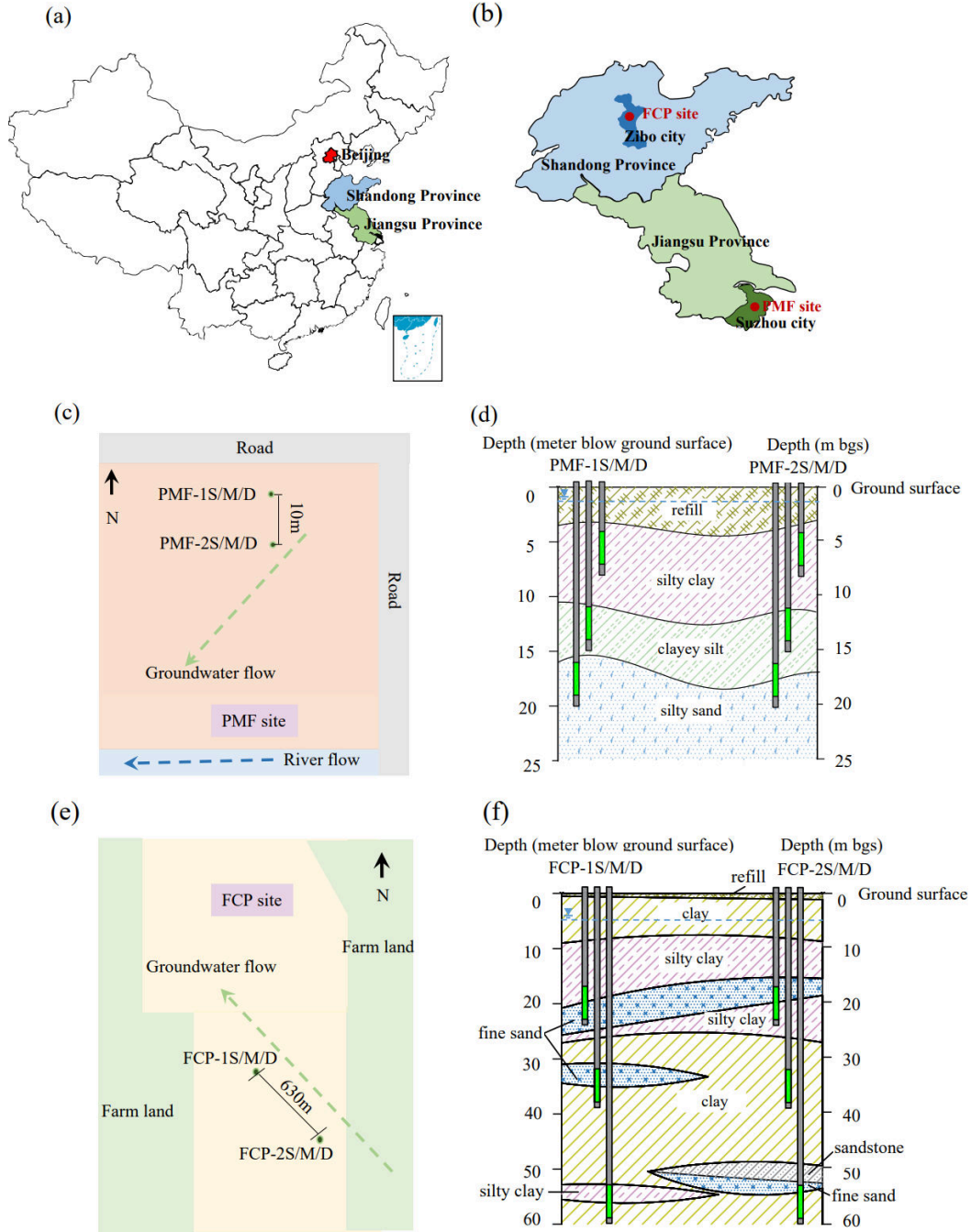
Fig. 1. Site locations (a, b), and layouts of groundwater monitoring wells and hydrogeological strata at the PMF (c, d) and FCP (e, f) sites.
