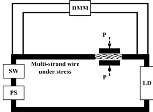
Fig. 5. Test 3, to examine changes in the resistance of wire as the connection is stressed by pressure (P).
