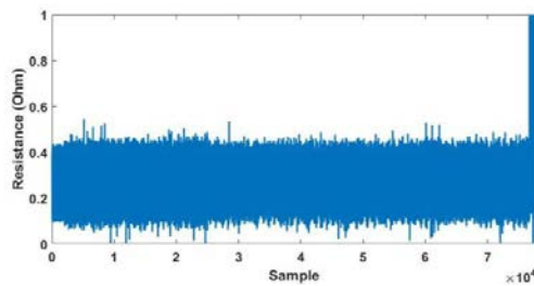
Fig. 10. Twisting the wire under test in a dead circuit, S_{2,2} . Meaningful changes in the resistance hardly can be detected.
