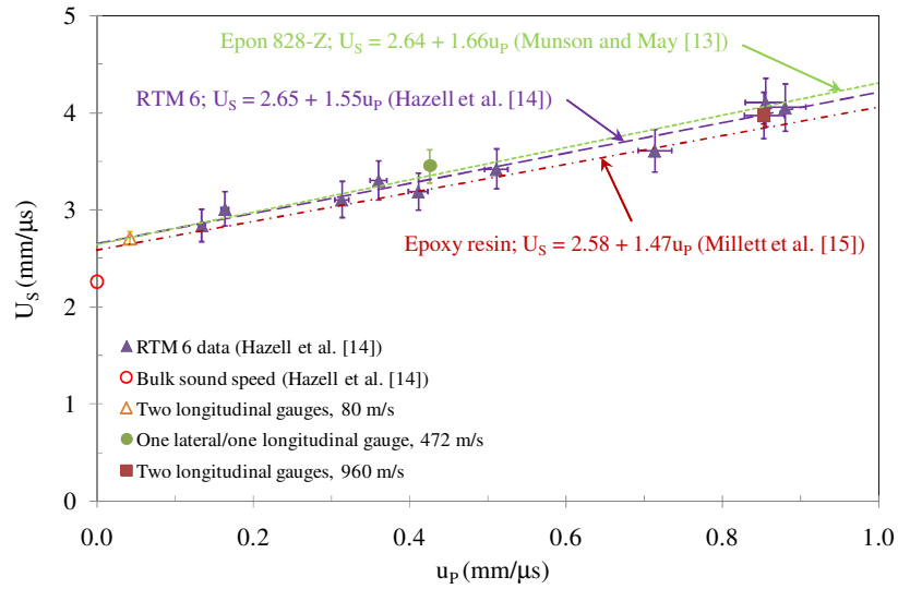
Fig. 5 U_S - u_P Hugoniot relationships for Epon 828-Z [13], RTM 6 [14] and a bespoke epoxy resin [15].
