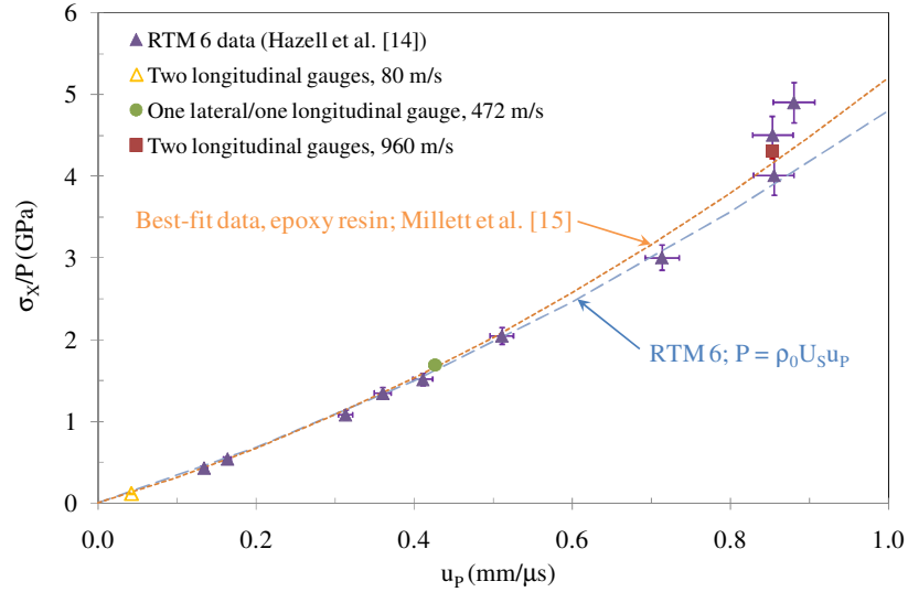
Fig. 6 \sigma_X - u_P Hugoniot relationships for RTM 6 [14] and a bespoke epoxy resin [15].
