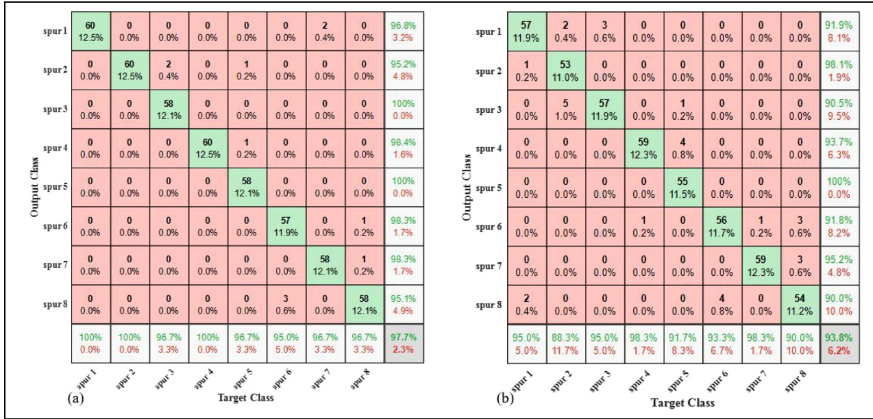
Figure 7. Confusion matrix of: (a) CNN-1 and (b) CNN-2.
