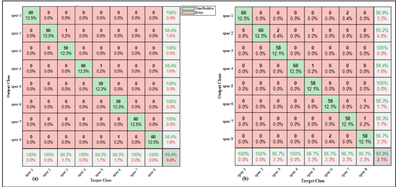
Figure 9. Proposed model's confusion matrix: (a) BECNN-SVM and (b) BECNN-DT.
