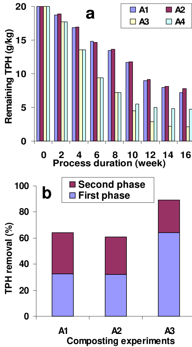
Fig. 3. (a) Residual TPH over the process duration in the composting bioreactors; and (b) percentages of TPH removal over the FP and SP duration in the composting bioreactors
