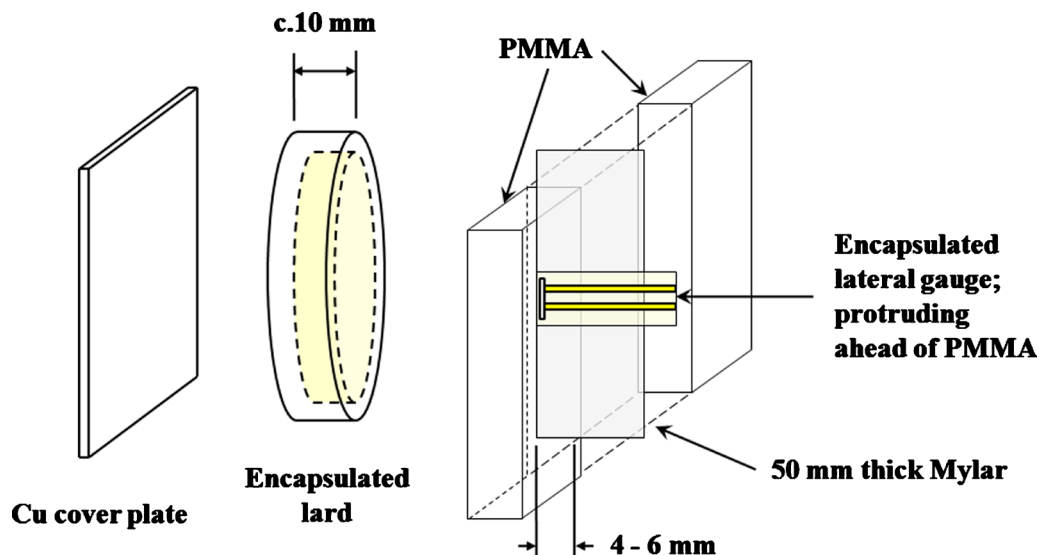
FIG. 2. (Color online) Schematic illustration of key elements of lard-encapsulation system (casting holes not-shown).
