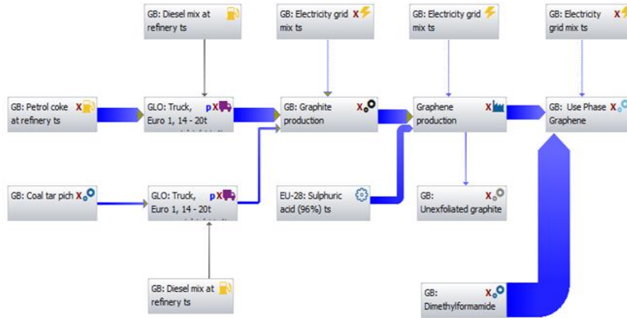
Fig. 8. LCA model of graphene capturing the cradle to gate approach
