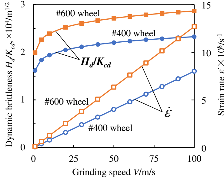
Fig. 9: Variation of the dynamic brittleness H_d/K_{Cd} and strain rate with grinding speed
