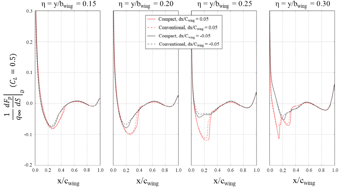
b) Axial cuts along the wing span: \eta = y/b_{\text{wing}} = 0.15, 0.20, 0.25 and 0.3 .
