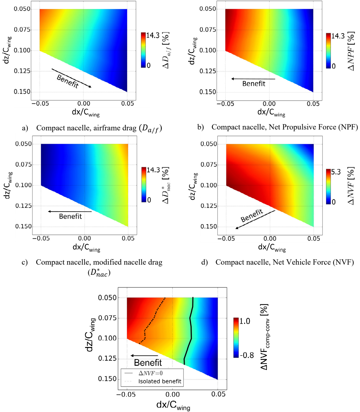
Figure 4: Installation maps at the cruise condition.
