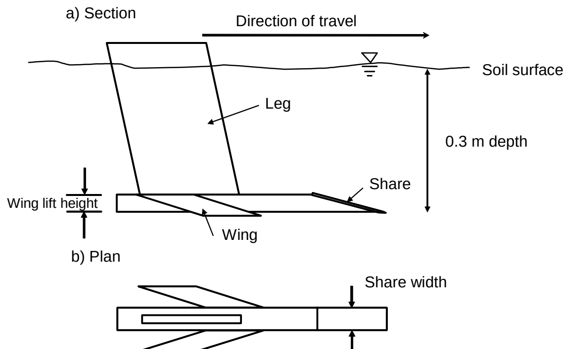
Figure 1. a) Section and b) plan view of a winged tine of the type used to loosen compacted soil. The tine is pulled through the soil behind a tractor.
