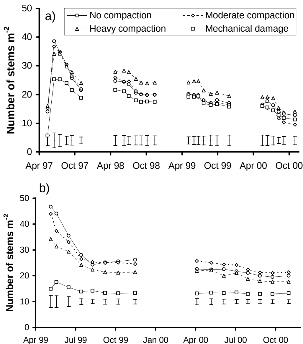
Figure 5. The effect of compaction and mechanical damage treatments on stem density on a) clay loam and b) sandy loam. Bars indicate the standard error of the difference between treatment means (10 d.f.; 3 d.f. for sandy loam during 2000).
