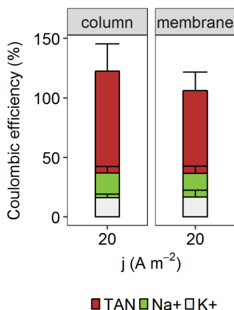
Fig. 3 Average ( \pm SD) coulombic efficiency (%) at 20 A m -2 for monovalent ions in steady state for both column (left) and membrane (right) stripping reactors. The coulombic efficiency is defined as the amount of cations extracted from the anolyte over the cation exchange membrane compared to the amount of applied electrons. The sum of all ions makes up for a 100% efficiency indicating electromigration. (n = 3)
