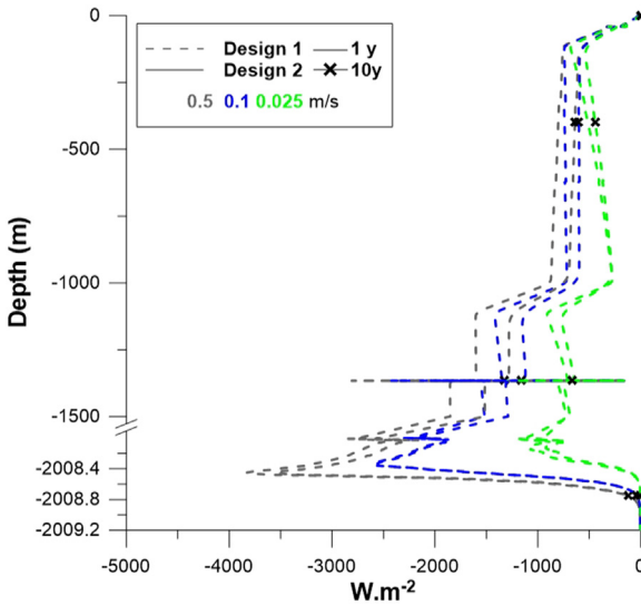
Fig. 13. Heat flux on the external well bore for Design 1. The vertical depth is arbitrary stopped at -2009 m to analyse the local variations. Zero heat flux values are calculated from -2009 m to -2070 m.
