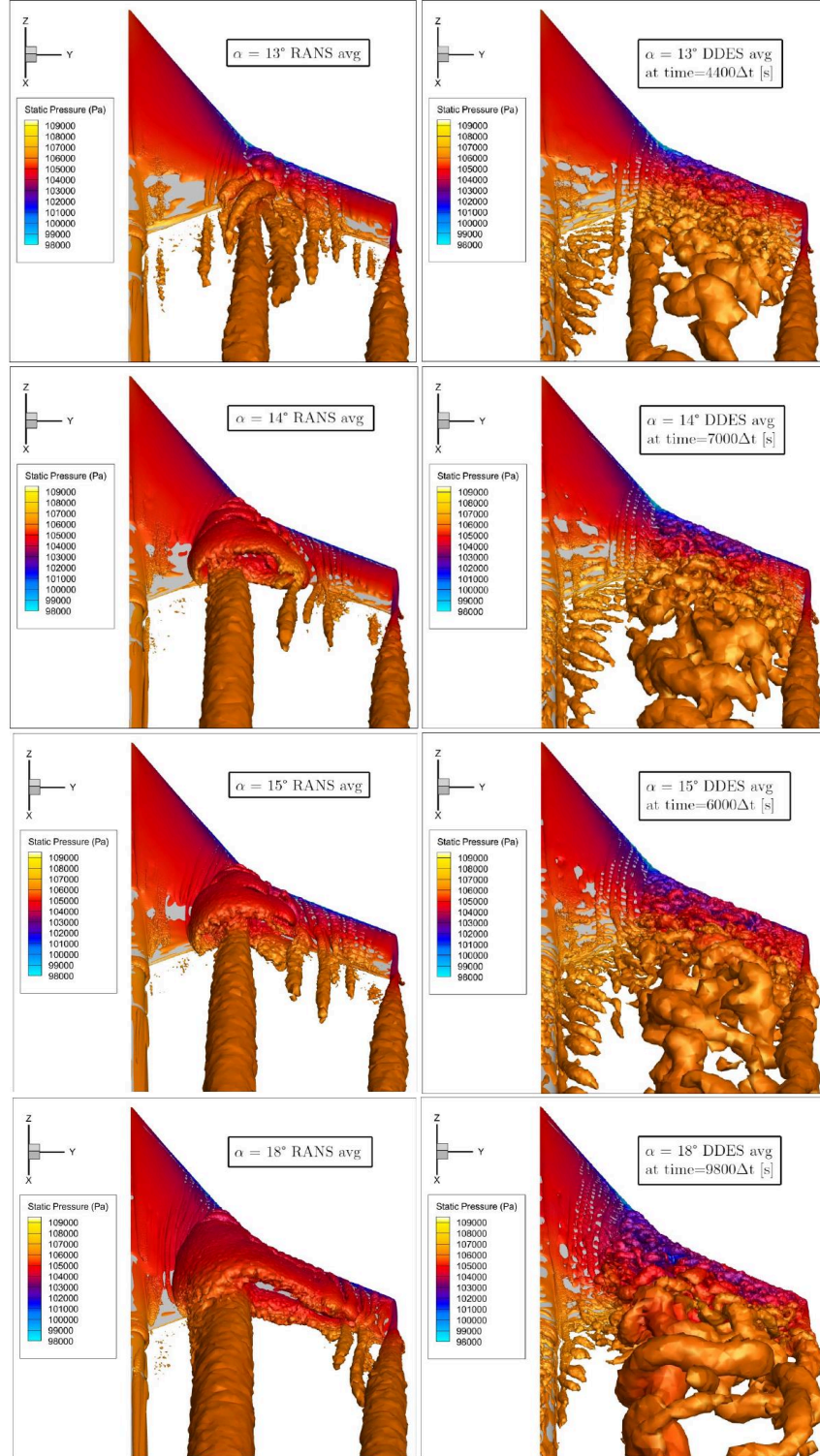
Fig 11: Comparison of the predicted Q -criterion iso-surface ( Q=20,000 flooded by static pressure contours) for the flow over the upper surface at the CL(average) condition. M = 0.2 , \alpha = 13^\circ\text{-}18^\circ , Re\bar{c} = 2.5 \times 10^6 .
