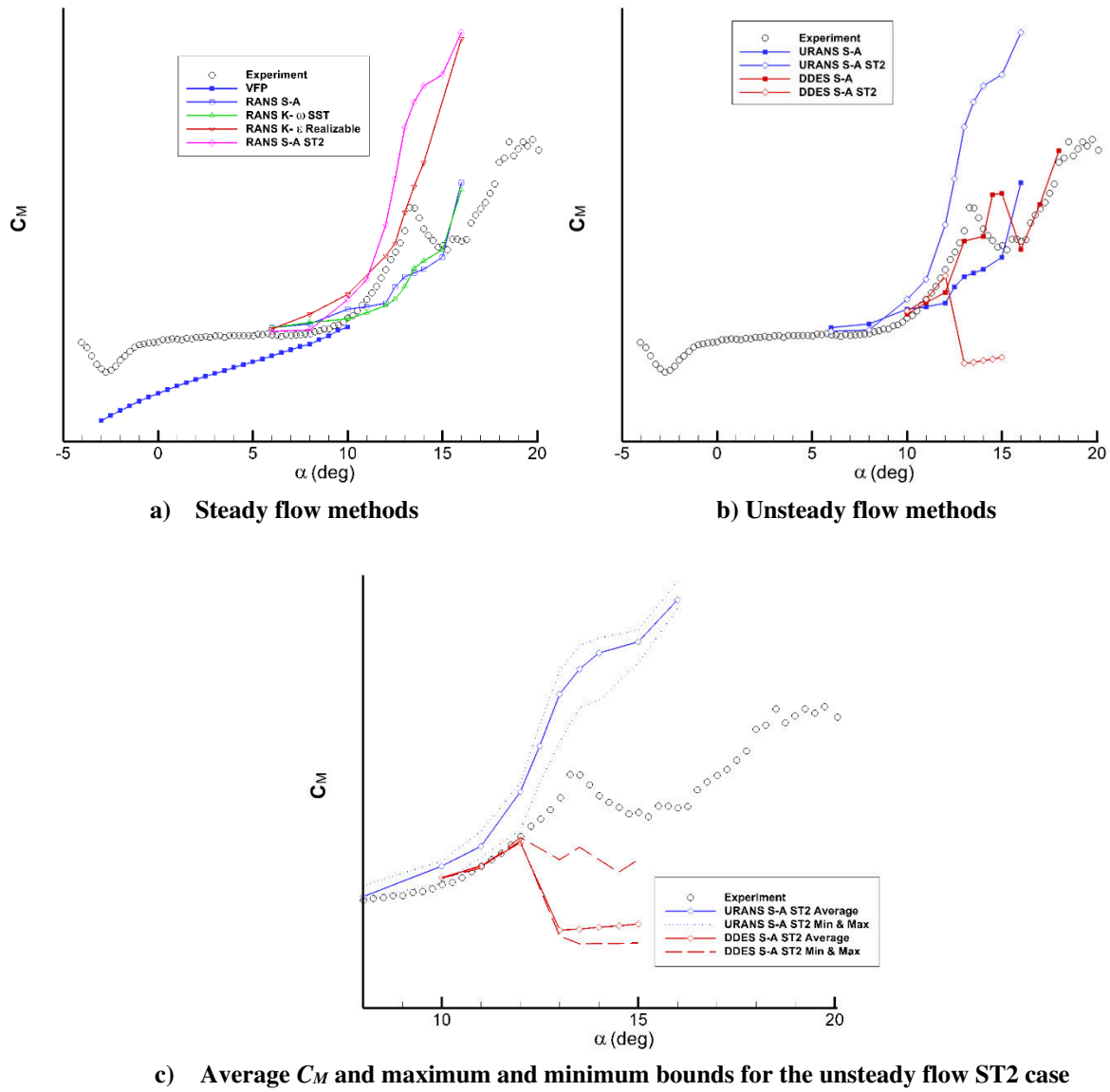
Fig 5: Comparison of C_M versus \alpha for the various CFD methods assessed. M = 0.2 , Re_c = 2.5 \times 10^6 .
