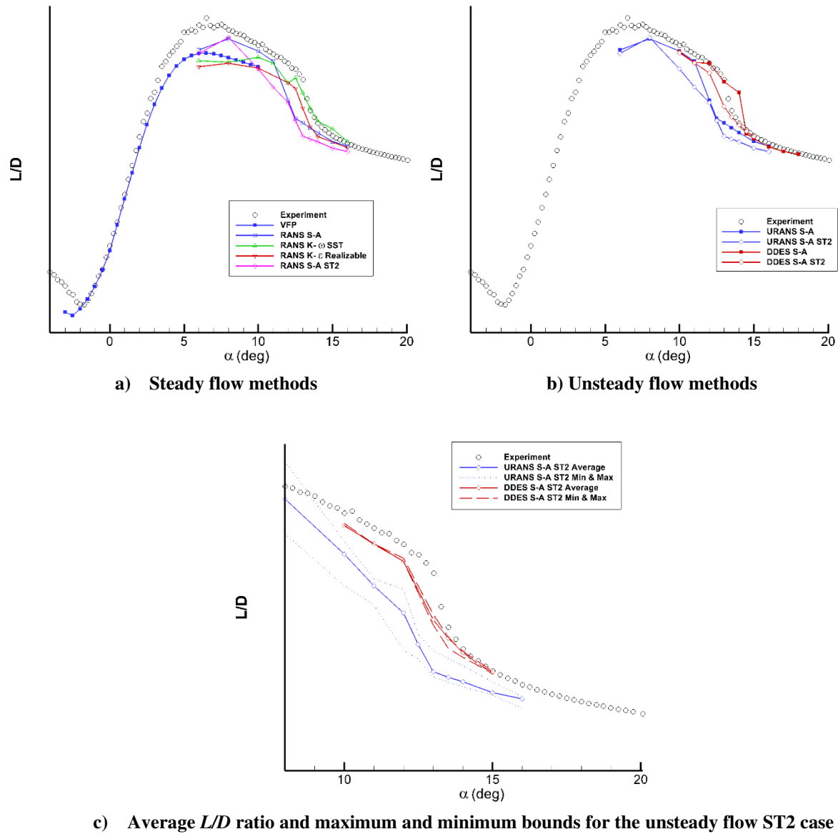
Fig 6: Comparison of L/D ratio versus \alpha for the various CFD methods assessed. M = 0.2 , Re_c = 2.5 \times 10^6 .
