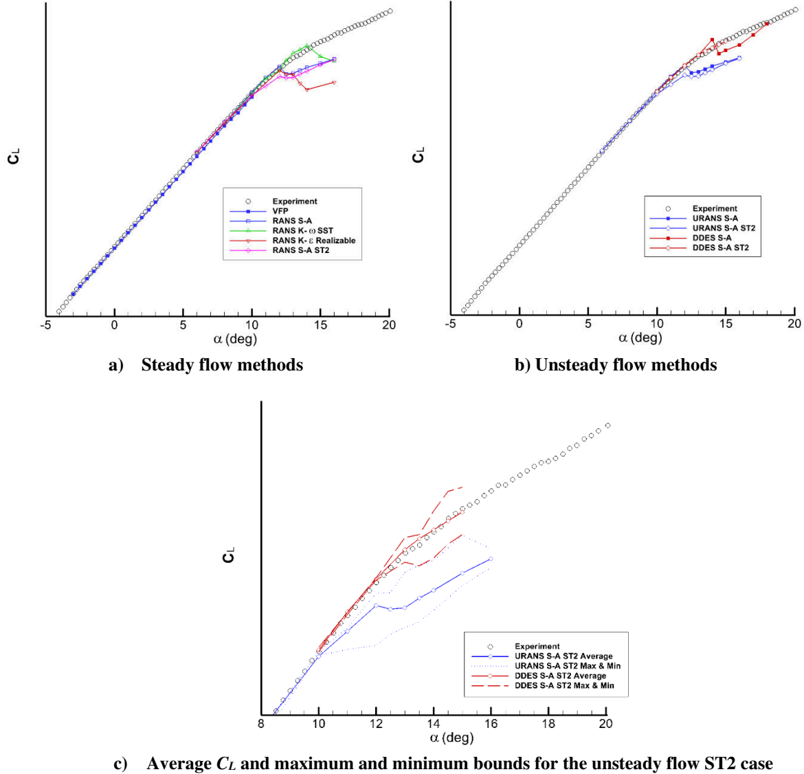
Fig. 3: Comparison of C_L versus \alpha for the various CFD methods assessed. M = 0.2 , Re_c = 2.5 \times 10^6 .
