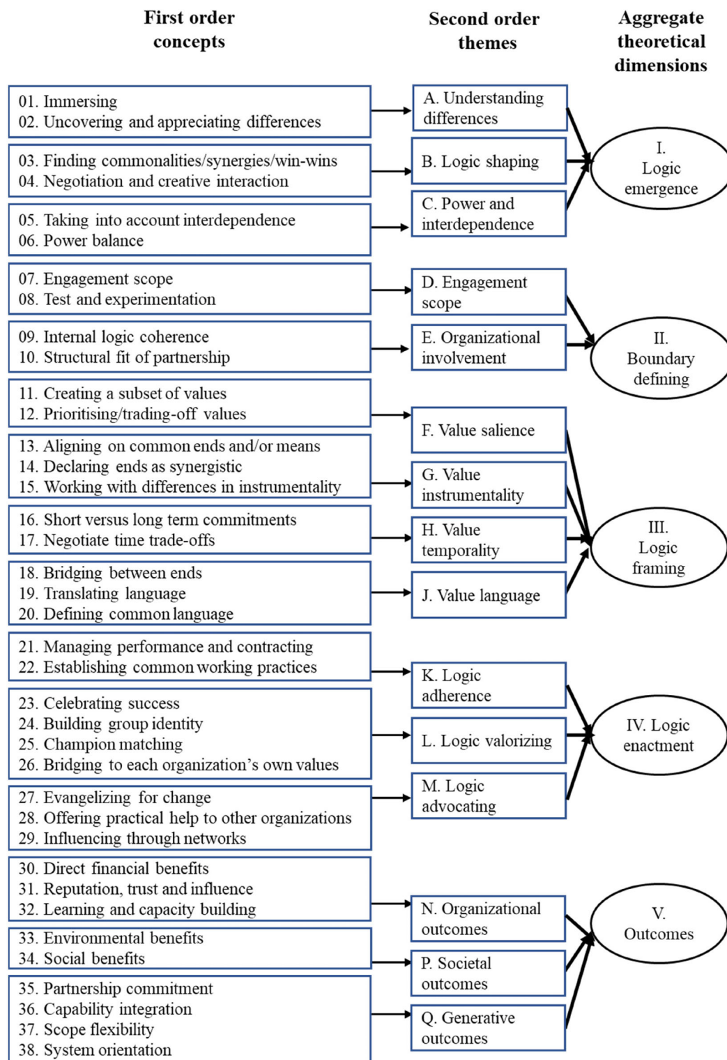
FIGURE 1 Data structure.
