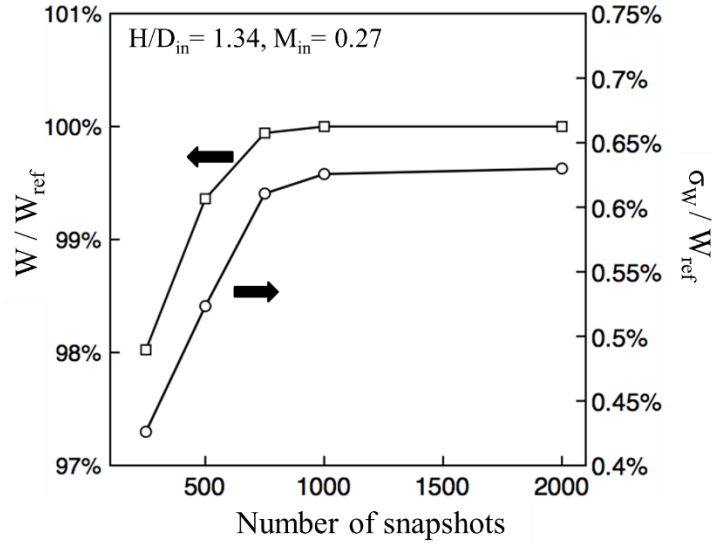
Fig. 5 Effect of number of snapshots on W / W_{ref} and \sigma_w / W_{ref} for Duct 1 ( H/D_{in} = 1.34 ) at M_{in} = 0.27 .
