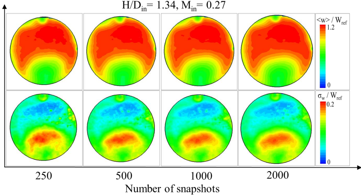
Fig. 4 Effect of number of S-PIV snapshots on spatial distributions of \langle w \rangle / W_{ref} and \sigma_w / W_{ref} for Duct 1 ( H/D_{in} = 1.34 ) at M_{in} = 0.27 .
