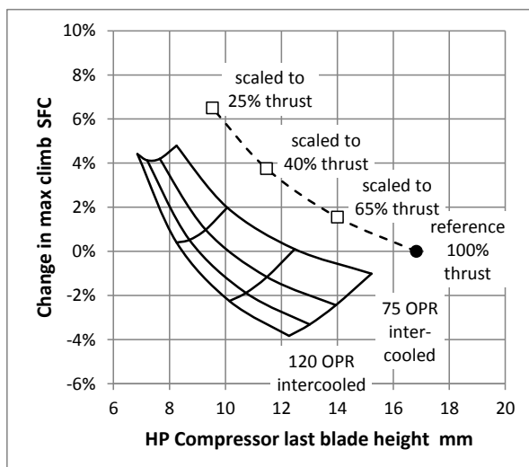
Figure 18 Effect of HP compressor last blade height and max climb OPR on max climb SFC for engines with 75% intercooler effectiveness v. the best conventional engines
