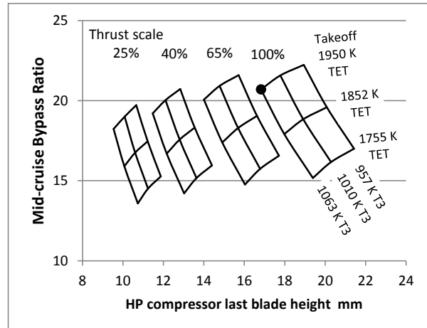
Figure 15 The effect on mid-cruise bypass ratio of scaling the reference engine and designing it for different hot day takeoff temperature limits for T_3 and TET
