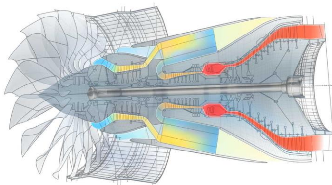
Figure 1 Schematic diagram of an intercooled engine with a low-speed LP turbine and a direct-drive fan
