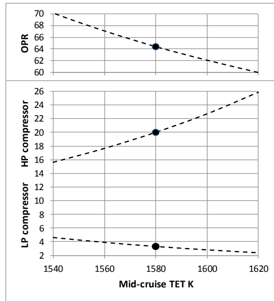
Figure 7 Effect on compressor pressure ratios of varying the fan/LP compressor work-split at cruise assuming constant compressor efficiencies
