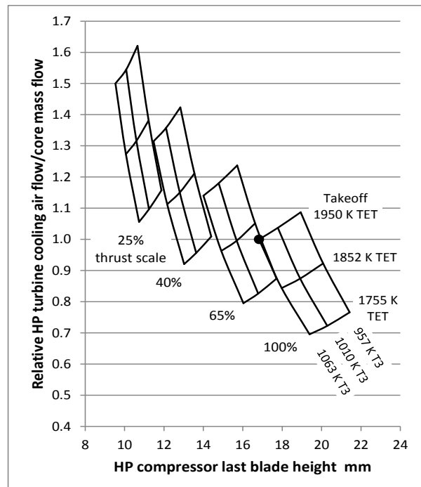
Figure 13 The effect on reference engine cooling flows of thrust scaling with different T_3 and TET limits at hot day takeoff v. HP compressor last blade height
