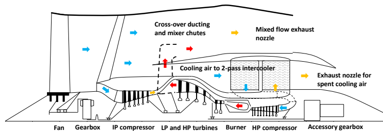
Figure 2 Schematic diagram of a reverse flow core intercooled turbofan aero engine arrangement
