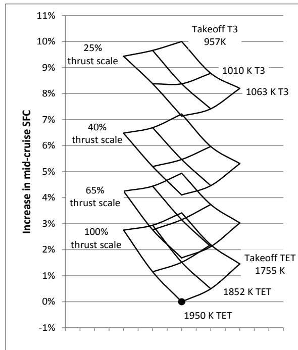
Figure 12 The effect on mid-cruise SFC of scaling the reference engine and designing it for various hot day takeoff temperature limits for T_3 and TET
