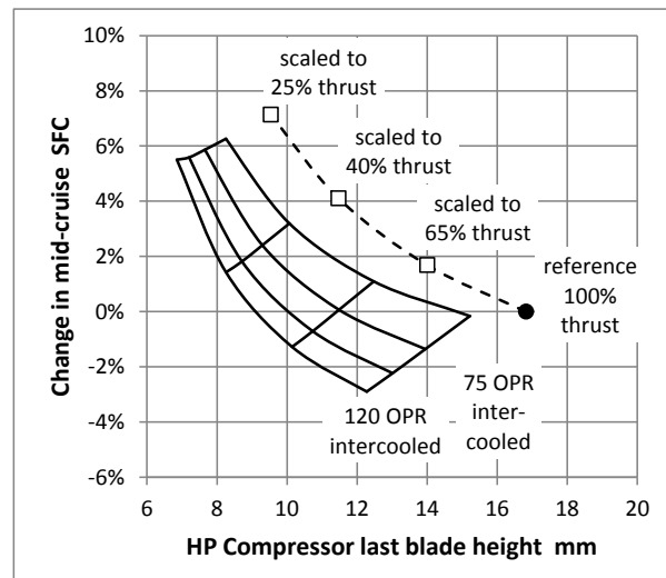
Figure 19 Improvements in mid-cruise SFC for intercooled engines from Fig. 18 with optimised mid-cruise intercooler effectiveness, OPR and TET v. the best conventional engines
