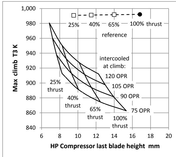
Figure 20 Max climb T3 for the conventional and intercooled engines from Fig. 18
