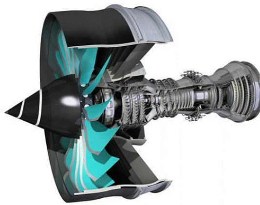
Figure 3 Rolls-Royce UltraFan™ engine concept having a variable-pitch geared fan
