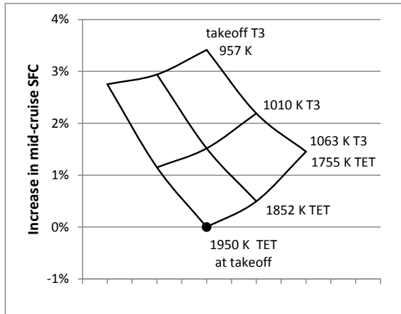
Figure 10 Effect of reducing hot day takeoff TET and T_3 on the reference engine mid-cruise SFC
