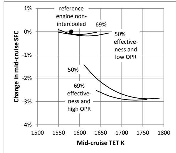
Figure 17 How mid-cruise SFC varies with TET and intercooler effectiveness for two different engines with 75 and 120 OPR at the max climb design point
