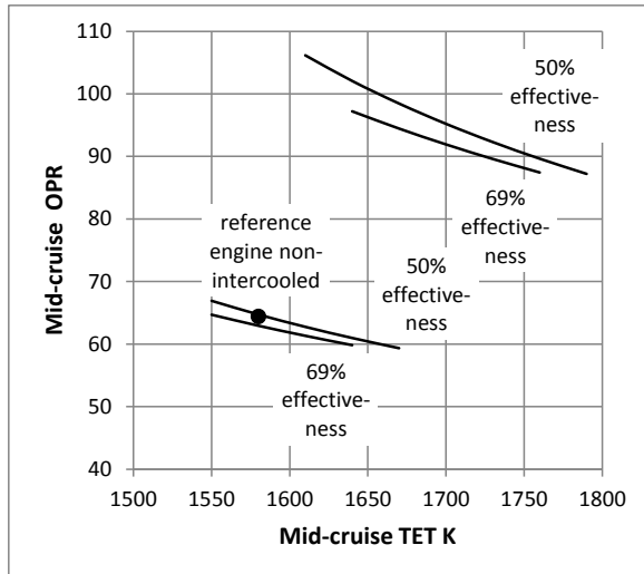
Figure 16 How mid-cruise OPR varies with TET and intercooler effectiveness for two different engines with 75 and 120 OPR at the max climb design point
