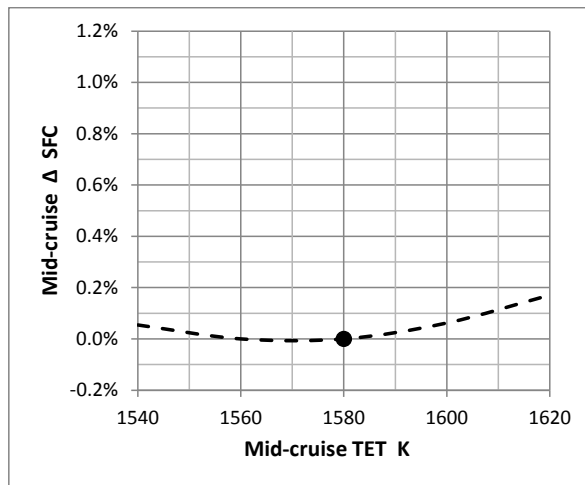
Figure 8 Effect on mid-cruise SFC of varying the fan/LP compressor work-split at constant component efficiency
