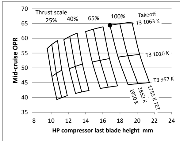
Figure 14 The effect on HP compressor blading and mid-cruise OPR of scaling the reference engine and designing it for different hot day takeoff temperature limits
