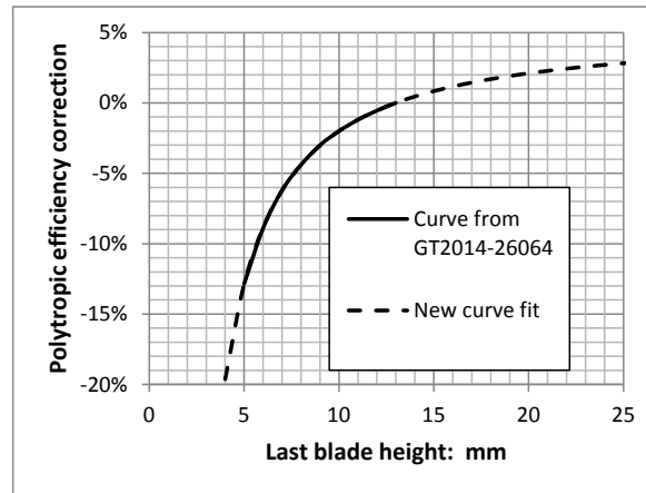
Figure 4 HP Compressor Correction to Polytropic Efficiency
