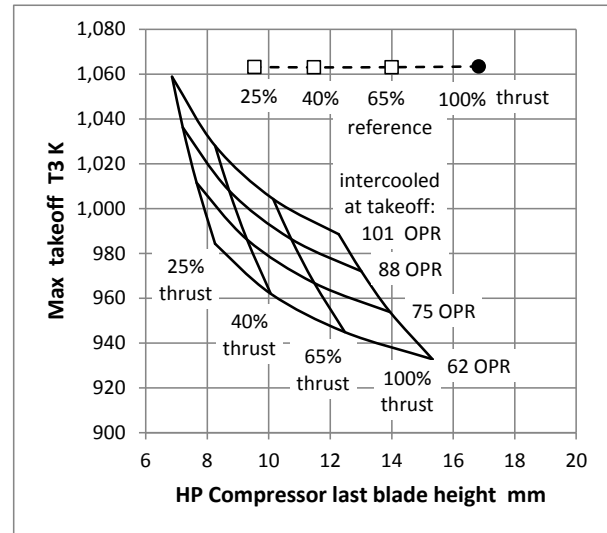
Figure 21 Max takeoff T3 for the conventional and intercooled engines from Fig. 18
