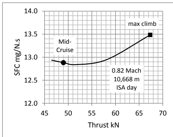
Figure 5 Reference 2050 turbofan SFC loop
