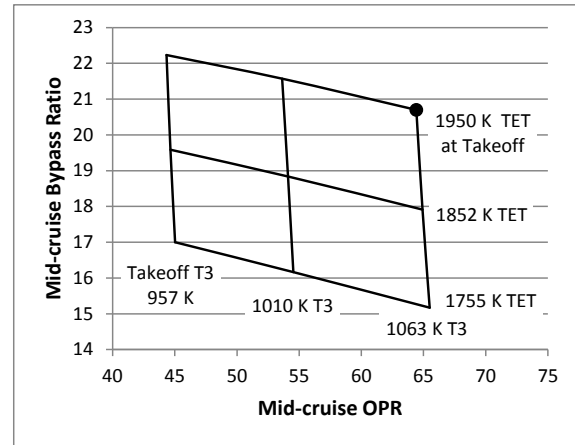
Figure 11 Effect of reducing hot day takeoff TET and T_3 on the reference engine mid-cruise OPR and bypass ratio
