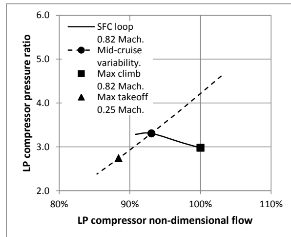
Figure 9 LP compressor altitude working line and the effect of varying the fan/LP compressor work-split
