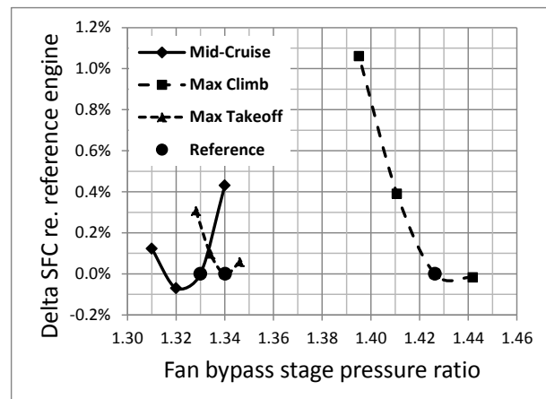
Figure 6 Effect of fan pressure ratio on SFC
