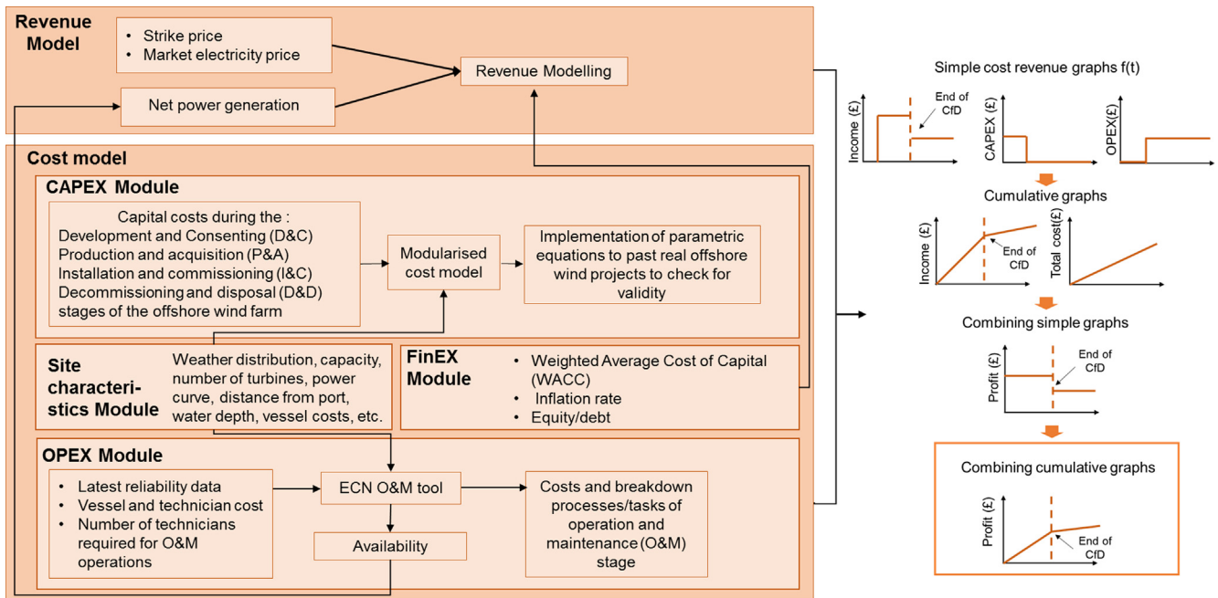
Fig. 1. Methodological framework.
