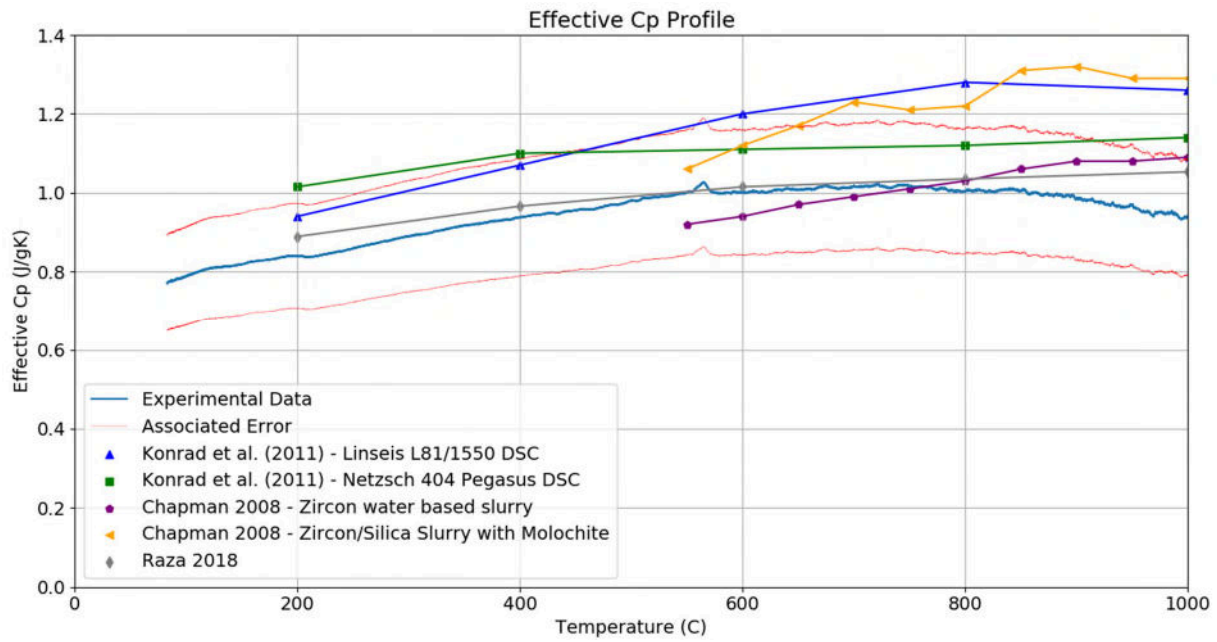
Figure 2. Comparative plot between the experimental C_p data and previous results from the literature as a function of temperature
