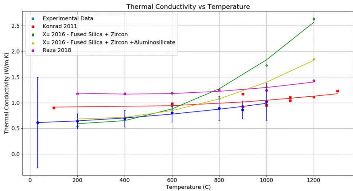
Figure 3. Comparative plot between the calculated thermal conductivity and thermal conductivity data published in literature sources as a function of temperature
