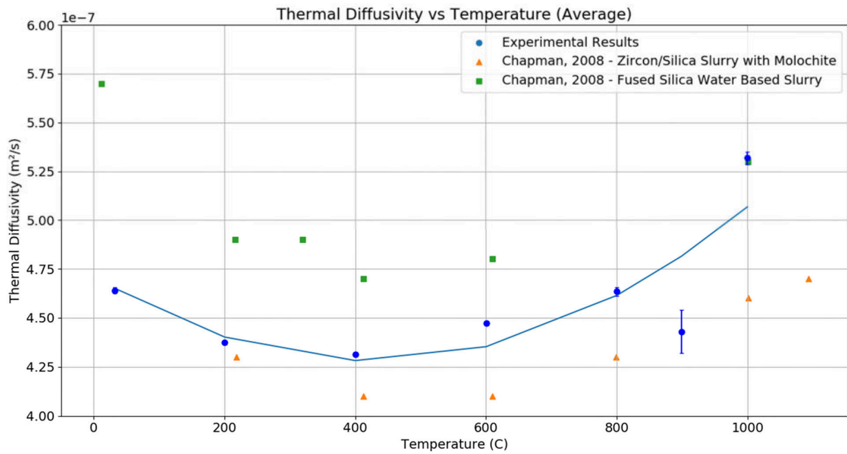
Figure 1. Comparative plot between the experimental thermal diffusivity profile and results published in literature as a function of temperature
