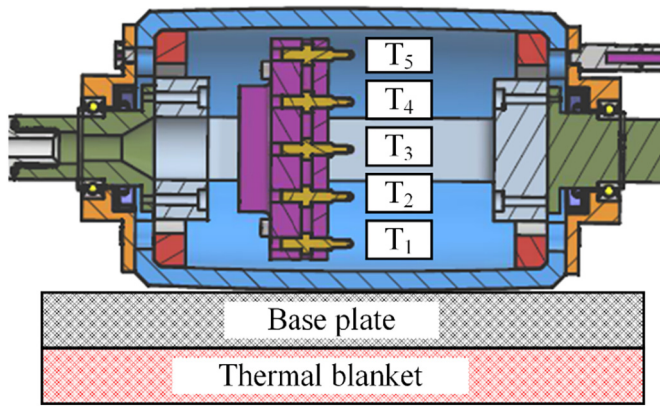
Fig. 8. Cross-sectioned roller probe assembly illustrating thermistor carriage with internal assembly structure within the roller probe and thermal blanket arrangement.
