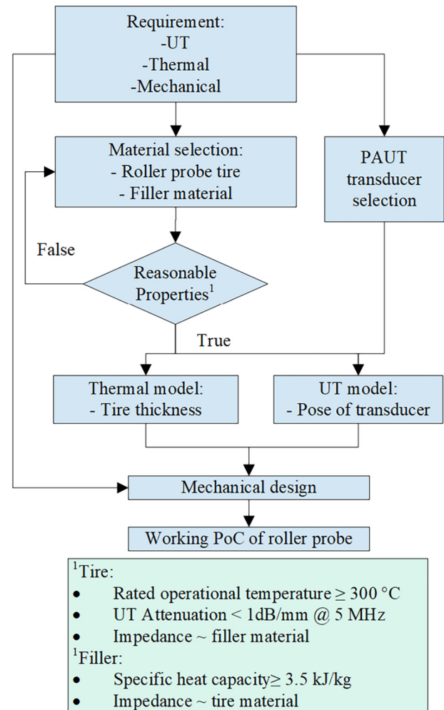
Fig. 3. Generic workflow of the roller probe development with ideal properties.
