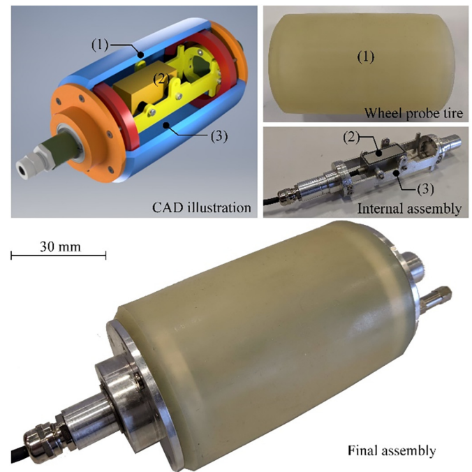
Fig. 7. Computer-aided design and physical assembly of the PAUT roller probe: (1) silicone tyre, (2) 5 MHz-64 element linear PAUT and (3) PAUT carrier.
