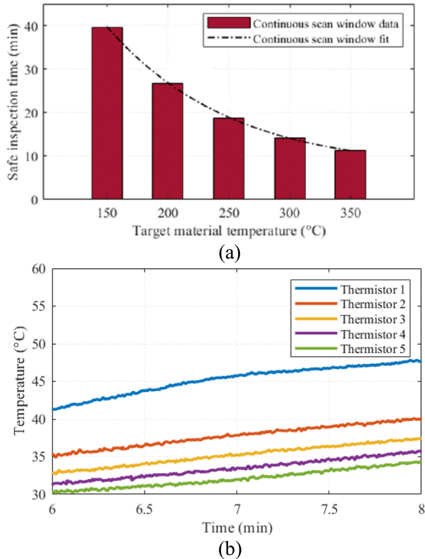
Fig. 9. (a) Continuous scan window of the liquid-filled roller probe for different base plate temperatures and (b) internal temperature distribution within the liquid domain.
