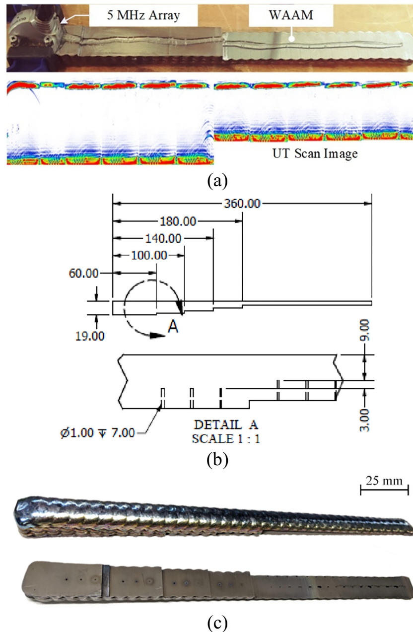
Fig. 10. WAAM calibration block. (a) Initial screening method and UT scan image of the extracted WAAM sample, (b) calibration block dimensions and (c) top and bottom view of the 26 mm wide WAAM calibration block.
