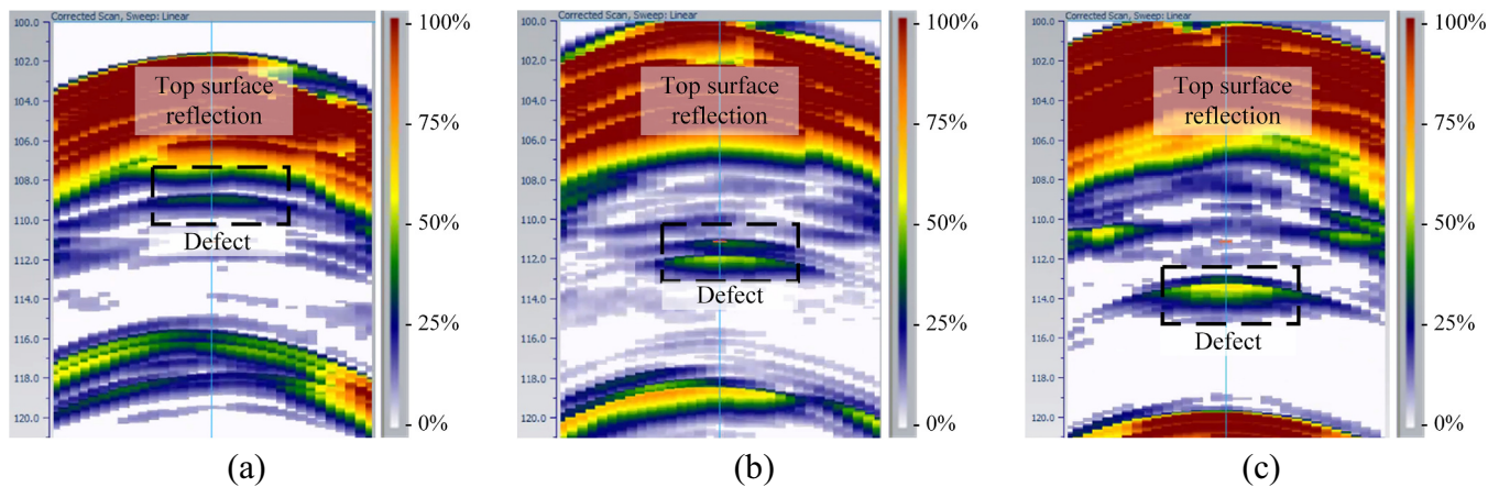
Fig. 12. BScan images of 1 mm Diameter FBHs located at (a) 6 mm, (b) 9 mm and (c) 12 mm depths.
