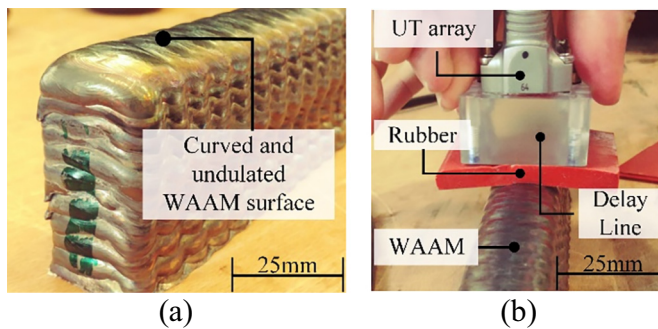
Fig. 2. (a) Laterally curved and the undulated surface of a straight WAAM wall and (b) rubber as a geometrically compliant interface.
