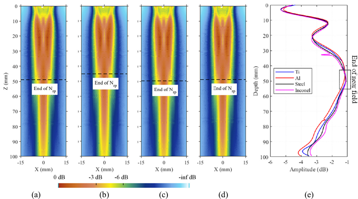
Fig. 5. (a)–(d) Acoustic energy map and end of near field within Ti, Al, Mild steel and Inconel and (e) UT wave energy fluctuation within each material in dB and region end of near field.
