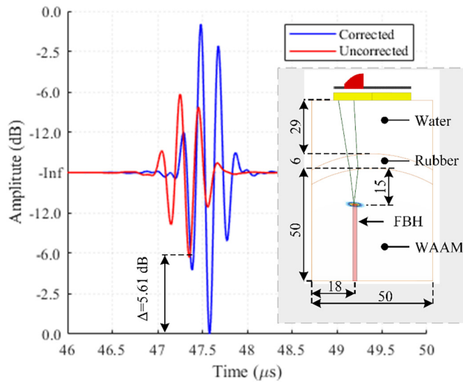
Fig. 6. Illustration of the ultrasound setup mimicking PAUT roller probe and maximum A-Scan signals correspond to FBH with corrected and uncorrected focal laws for the curvature of the simulated WAAM surface.
