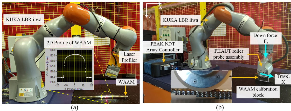
Fig. 11. (a) Quantification of WAAM lateral curvature using a 2D laser profiler and (b) experimental setup illustrating PAUT roller probe, array controller, Ti64 WAAM calibration block with 1 mm FBH and industrial robot with inbuilt force-torque control capability.
