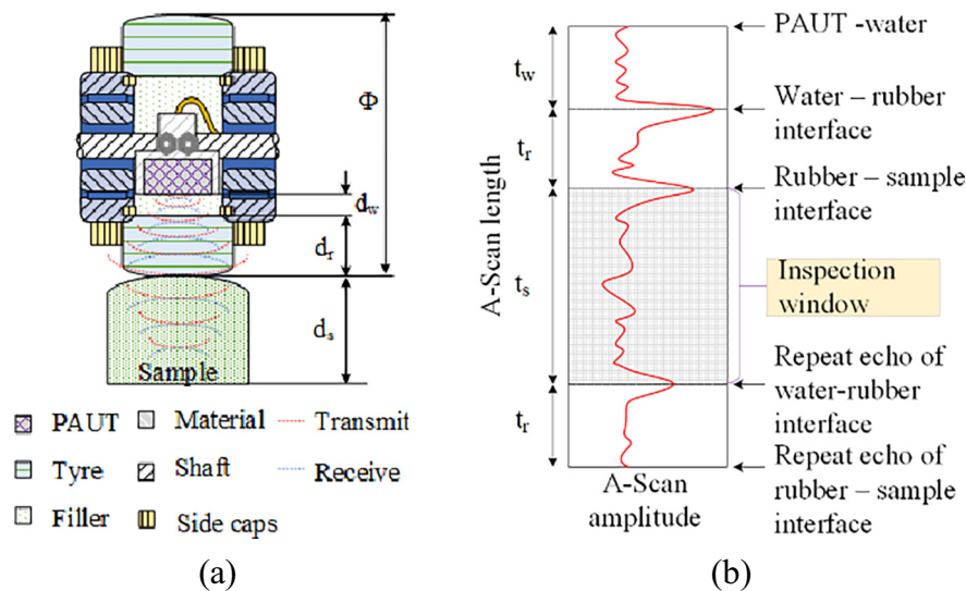
Fig. 4. (a) Schematic of the roller probe illustrating array configuration, positioning on a WAAM sample and indicative transmit-receive ultrasound wave and (b) A-Scan signal illustrating surface echoes.
