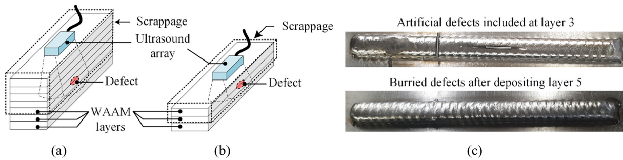
Fig. 1. UT inspection and scrappage due to (a) post-process inspection, (b) in-process inspection of WAAM components and (c) example WAAM component with intentional defects embedded at layer three and fully covered after depositing layer five.
