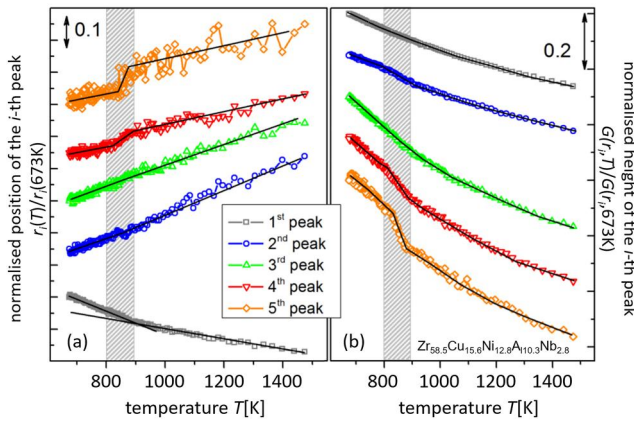
Figure 15. Kinks in the normalised position r_i(T)/r_i(673\text{ K}) and height G(r_i, T)/G(r_i, 673\text{ K}) of the first five peaks ( i = 1 \dots 5 ) during an LLC (hatched region) of Vitreloy 106a ( \text{Zr}_{58.5}\text{Cu}_{15.6}\text{Ni}_{12.8}\text{Al}_{10.3}\text{Nb}_{2.8} ) upon cooling (reproduced with permission from ref. [18]). Curves are shifted on the y-axes for clarity and the solid lines are a guides to the eyes. Note the combined occurrence of kinks and non-linear behaviour.
