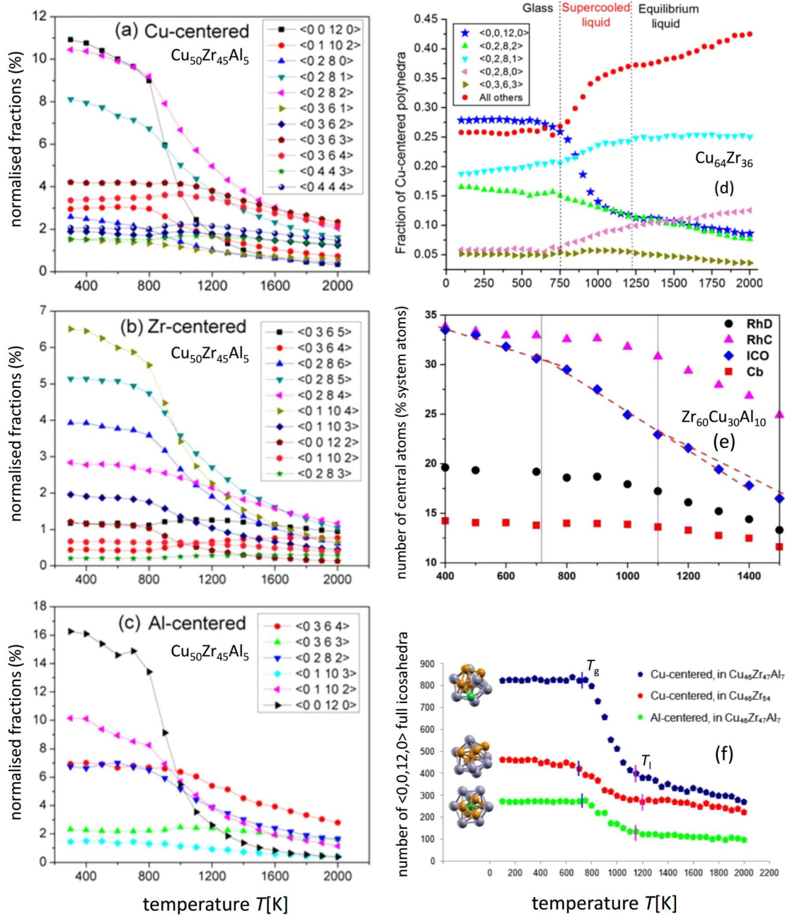
Figure 12. Results from MD simulations of various metallic glass forming liquids upon cooling. A rapid acceleration of cluster formation in the undercooled regime is clearly visible. This is especially the case for clusters with icosahedral-like symmetry. In (a), (b), (c), (d) and (f) so called Voronoi indices [168,169] are given where \langle 0,0,12,0 \rangle relates to perfect icosahedral symmetry, i.e. central atoms enclosed by Voronoi polyhedra (VP) with 12 pentagonal faces. (a–c) Shows the cluster evolution around the different elemental species in \text{Cu}_{50}\text{Zr}_{45}\text{Al}_5 (reproduced with permission from ref. [170] ). For \text{Cu}_{64}\text{Zr}_{36} the growth of the \langle 0,0,12,0 \rangle VP on the expense of clusters with other symmetries is highlighted in (d, reproduced with permission from ref. [171,172] ). In (e) cluster populations with rhombic dodecahedral (RhD), icosahedral (ICO) and cuboctahedral (Cb) shapes as well as the sum of the population of RhD and Cb clusters (RhC) are shown for \text{Zr}_{60}\text{Cu}_{30}\text{Al}_{10} (reproduced with permission from ref. [45] ). A comparison of the population of \langle 0,0,12,0 \rangle clusters in \text{Cu}_{46}\text{Zr}_{47}\text{Al}_7 and \text{Cu}_{46}\text{Zr}_{54} is shown in (f, reproduced with permission from ref. [165] ). As in the experimentally obtained metrics (Figure 11) mainly continuous non-linear dependences of the populations between T_l and T_g are visible.
