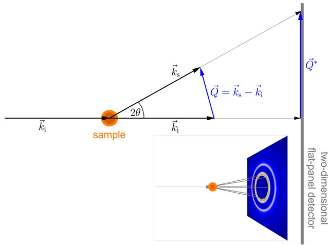
Figure 7. Geometry for elastic scattering methods in transmission. In case of a 2D flat-panel detector the scattering vector \vec{Q} has to be calculated from its projected version \vec{Q}^* . The scattering vector \vec{Q} “translates” the incident wavevector \vec{k}_i to the wavevector \vec{k}_s of the wave scattered elastically at scattering angle 2\theta , where |\vec{k}_s| = k_s = k_i = |\vec{k}_i| . The inset (adapted from ref. [108] ) sketches a slanted view on the geometry illustrating the relation of sample, beams and diffraction pattern.
