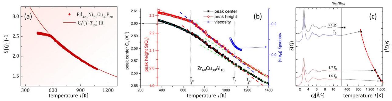
Figure 11. Non-linear temperature dependence of structural metrics in reciprocal space for different metallic glasses. A Curie-Weiss-like behaviour has been proposed recently and was fitted to the experimentally obtained height S(Q_1) - 1 of the first peak of the structure factor of \text{Pd}_{42.5}\text{Ni}_{7.5}\text{Cu}_{30}\text{P}_{20} (a, reproduced from ref. [37]). For the height S(Q_1) and position Q_1 of \text{Zr}_{60}\text{Cu}_{30}\text{Al}_{10} the continuous non-linear shape has been approximated discontinuously using two linear functions each whose intersection was associated with a stark increase in the viscosity \eta(T) (b, reproduced with permission from ref. [45]). A lack of data for wide T regions severely hampers a correct fit as in the case of \text{Ni}_{62}\text{Nb}_{38} (c, adapted with permission from ref. [161]) but again allows for a non-linear dependence over the complete T region down to T_g as sketched by the red dashed line while originally a linear approximation [161] was used for the high- T region only.
