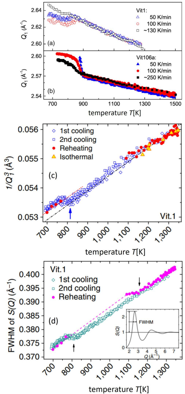
Figure 14. Kinks in structural metrics in reciprocal space during supposed LLCs and their temperature dependence. (a) The position Q_1 of the first peak of S(Q) of Vitreyloy 1 ( \text{Zr}_{41.2}\text{Ti}_{13.8}\text{Cu}_{12.5}\text{Ni}_{10}\text{Be}_{22.5} ) for three different cooling rates (reproduced with permission from ref. [163]). (b) the same for Vitreyloy 106a ( \text{Zr}_{58.5}\text{Cu}_{15.6}\text{Ni}_{12.8}\text{Al}_{10.3}\text{Nb}_{2.8} ) (reproduced with permission from ref. [163]). (c) 1/Q_1^3 (which is supposed to be a microscopic measure (esp. MRO) of the volume of the alloy) for Vitreyloy 1 (reproduced with permission from ref. [17]). (d) FWHM \Gamma(T) of the first peak of S(Q) of Vitreyloy 1 showing indications (marked by arrows) of a hysteresis (reproduced with permission from ref. [17]).
