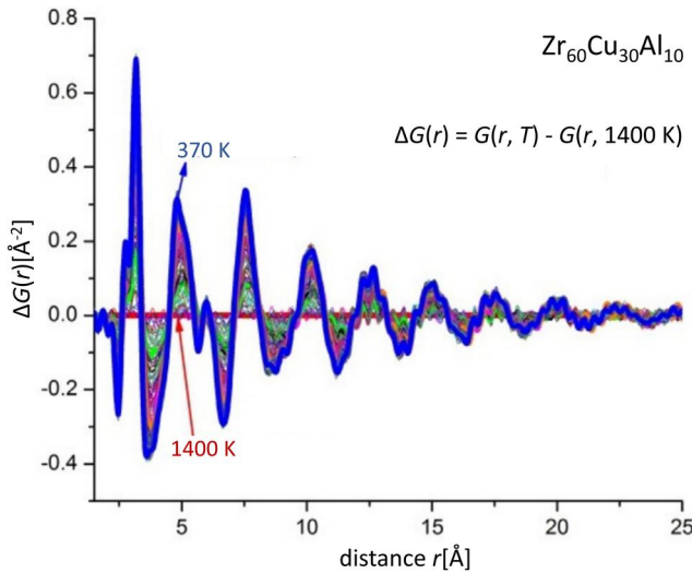
Figure 13. The function \Delta G(r, T) = G(r, T) - G(r, 1400 \text{ K}) for \text{Zr}_{60}\text{Cu}_{30}\text{Al}_{10} shows the transfer of atoms from the anti-shells to the shells upon undercooling, i.e., an increasing height of the peaks of \Delta G(r, T) accompanied by a decreasing depth of the troughs (reproduced with permission from ref. [45]).
