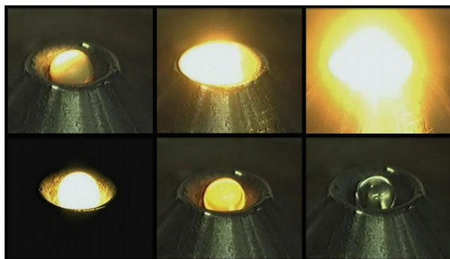
Figure 5. In-situ vitrification in a CNL setup showcased for an oxide melt (reproduced from ref. [11]). From top left to bottom right, the sample is heated and melted and subsequently vitrifies during cooling.
