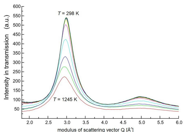
Figure 2. Intensity distribution I(Q) acquired using high-energy synchrotron X-ray diffraction in transmission at various temperatures for the first reported in-situ monitoring of the complete pathway from the equilibrium liquid down to the glass for metallic alloys ( \text{Pd}_{40}\text{Cu}_{30}\text{Ni}_{10}\text{P}_{20} , T_l = 864 K, T_g = 569 K) [33] (reproduced with permission from ref. [34] ).
