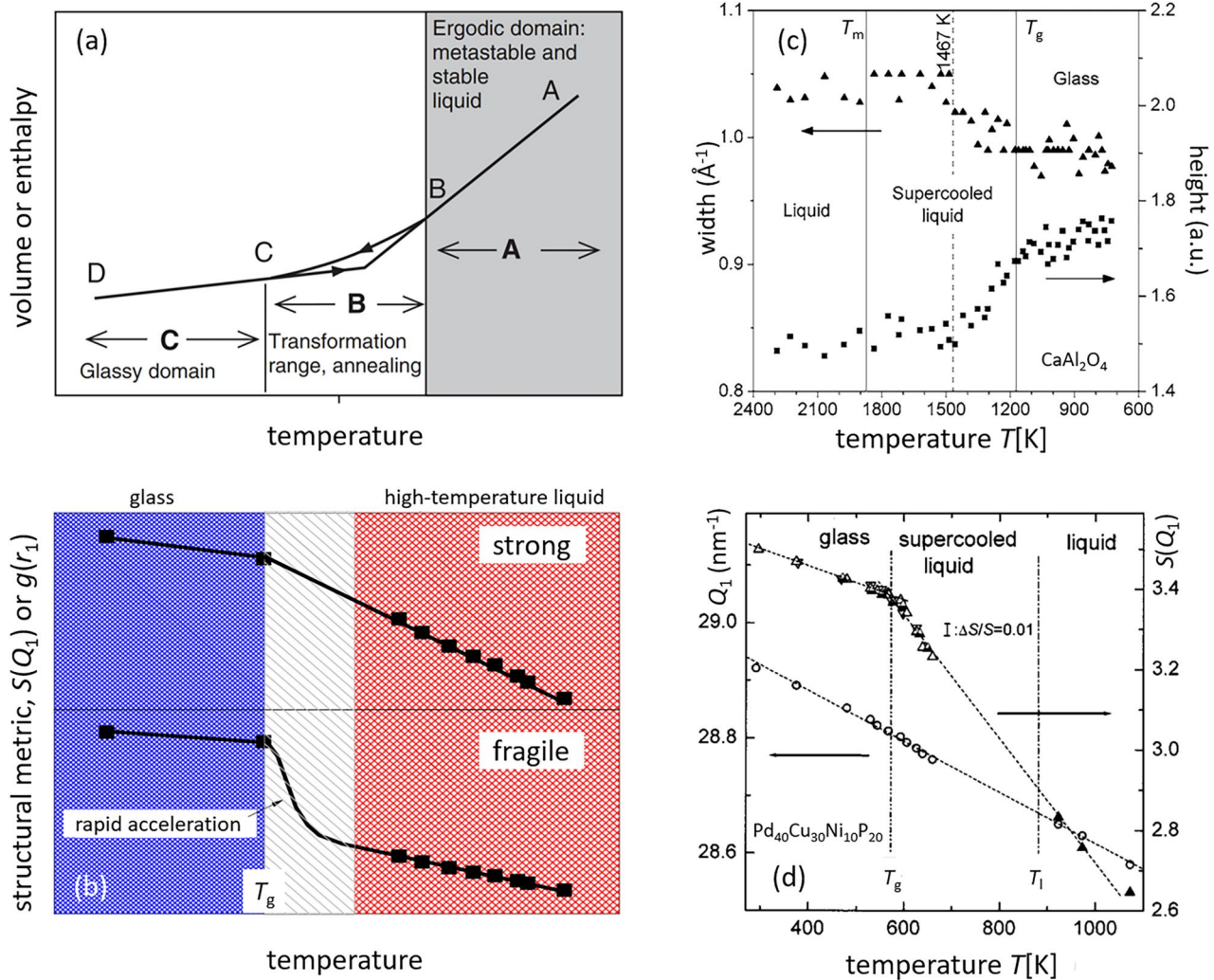
Figure 16. The pathway of liquids to vitrification can be separated into three different regimes. This subdivision is not unique and not agreed upon. Parallels to Angell's three domains of interest [31,215] can be drawn (a, adapted with permission from ref. [31] ) Mauro et al. (cf., e.g., ref. [160] ) hinted at three regimes, where the evolution of structural metrics in the region between high-temperature liquid and glass supposedly depends on the materials fragility (b, adapted with permission from ref. [160] ) Three regimes have also been pointed out for oxide melts (c, here \text{CaAl}_2\text{O}_4 adapted with permission from ref. [19] mind the flipped temperature scale). A possible LLC in the undercooled ("supercooled") regime ( T_{\text{LLC}} = 1467 \text{ K} ) and not T_m (or T_1 ) maybe the actual border of the first two regimes on cooling. Three regimes (glass, undercooled ("supercooled") liquid and liquid) have also been discussed for heating experiments (d, here \text{Pd}_{40}\text{Cu}_{30}\text{Ni}_{10}\text{P}_{20} , note how position Q_1 and height S(Q_1) are affected very differently across the glass transition; adapted with permission from ref. [35] ).
