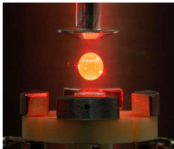
Figure 4. Electrostatic levitation exemplified for 0.6 g of liquid \text{Ti}_{39.5}\text{Zr}_{39.5}\text{Ni}_{21} (centre) at 1150 K (reproduced with permission from ref. [71] ).
