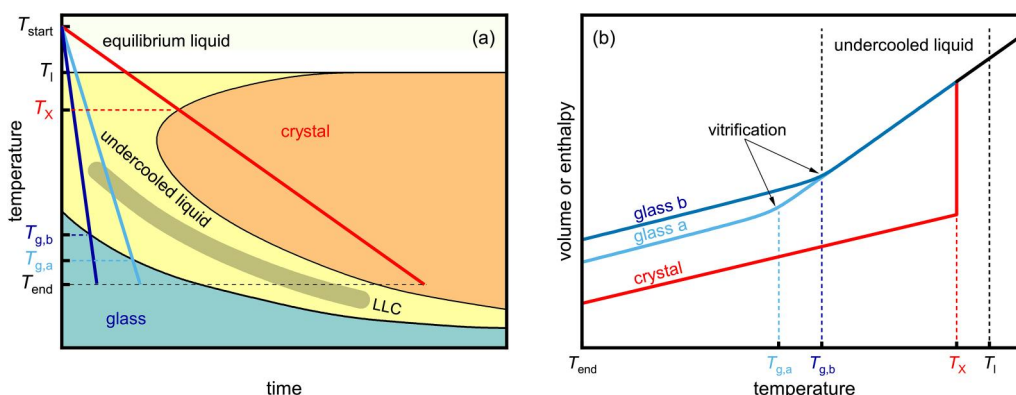
Figure 1. Schematic time-temperature-transformation (TTT) diagram of a model alloy quenched from T_{\text{start}} (well above the liquidus temperature T_l or melting temperature T_m in case of a eutectic alloy) with three different cooling rates (a) and the temperature dependence of its volume or enthalpy at constant pressure (b). The model experiment ends at T_{\text{end}} . Depending on the cooling rate the (undercooled) liquid can crystallise at T_x (red) or vitrify at different glass transition temperatures T_{g,a} (light blue) or T_{g,b} (dark blue) yielding glasses with slightly different properties (it needs to be mentioned that T_x depends on the cooling rate as well and also differs from a T_x upon heating the glass). Pathway b passes through a possible liquid-liquid crossover (LLC). Its range of existence and transition region is often only insufficiently known and, therefore, only roughly sketched in (a) (shaded in grey). The effects of LLCs on the macroscopic sample volume are controversial [15–18] and have been omitted in (b).
