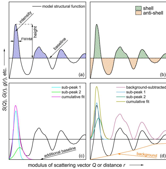
Figure 9. Possible ways of extracting peaks from a model structural function (black) and their fitting: (a) using the parts above a baseline, implied by the average of a structural function, (horizontal black line) only (peaks not necessarily to be fitted), (b) using portions above and below that baseline (especially in real space called NN shell and anti-shell), (c) defining an additional baseline for a fit (shown exemplarily for the first peak fitted by two sub-peaks), (d) removing a background (orange, determined by a set of linear functions) before fitting. In a) the definitions of intensity, height and FWHM are highlighted.
