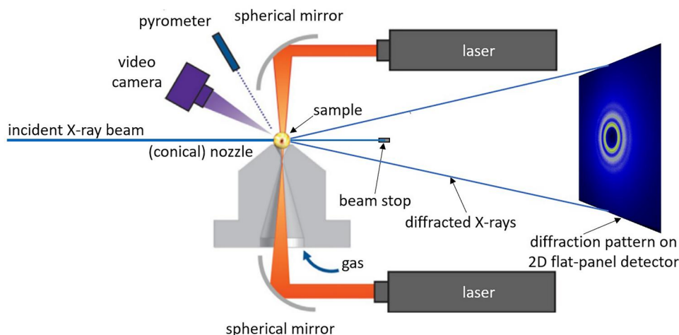
Figure 6. Schematic representation of conical-nozzle levitation and laser heating for synchrotron X-ray diffraction (adapted with permission from ref. [13]).
