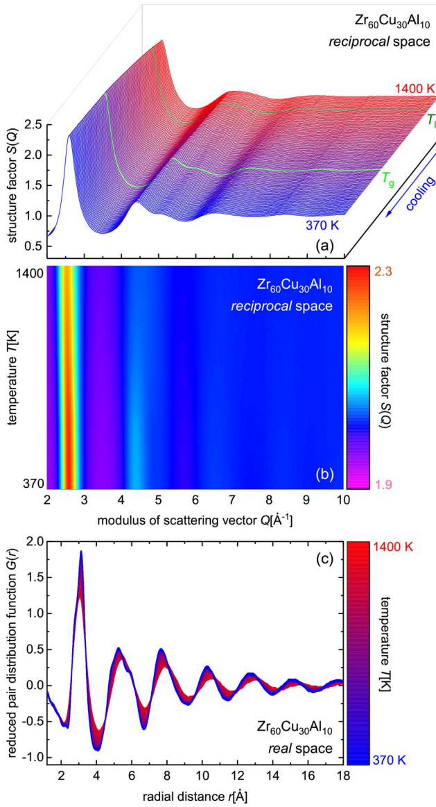
Figure 10. The evolution of structural functions along the pathway exemplarily for \text{Zr}_{60}\text{Cu}_{30}\text{Al}_{10} during cooling from 1400 K (red) to 370 K (blue) (data taken from ref. [45]). This also showcases different ways of visualising structural functions along the pathway. In (a) the T -dependence of the structure factor S(Q, T) is shown in a three-dimensional way as waterfall plot. Highlighted in green are the functions for the liquidus temperature T_l = 671 K and the glass-transition temperature T_g = 1207 K. Alternatively, in (b) the T -dependence of the structure factor S(Q, T) is shown as contour plot. The corresponding reduced pair-distribution functions G(r, T) are shown in (c) as 2D plot. Here T -dependent trends in the large amount of data can be followed with the help of the color coding.
