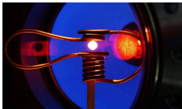
Figure 3. Electromagnetically levitated metallic droplet (centre) inside the coil responsible for levitation and heating (reproduced with permission from ref. [13] ).
