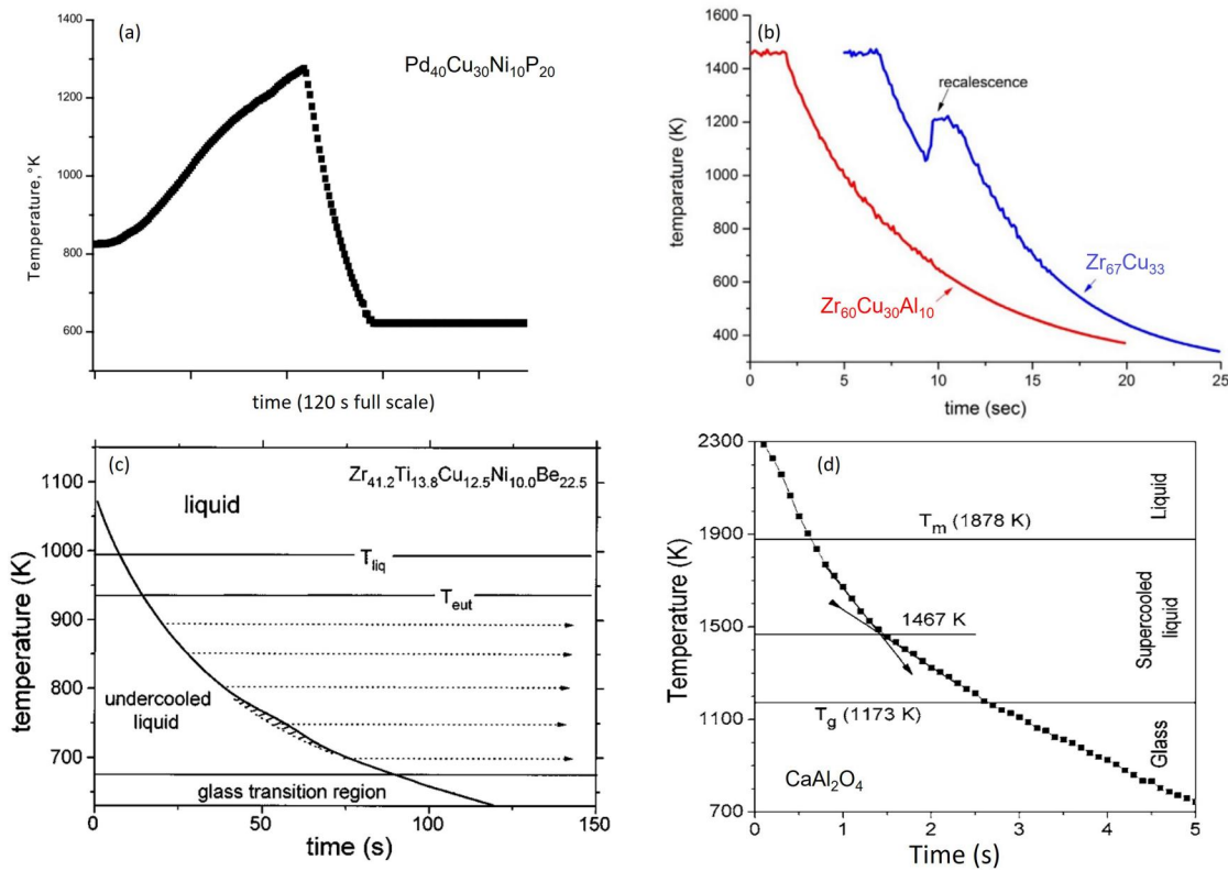
Figure 8. Examples of several T(t) functions ("cooling curves") and proposed interpretations. (a) The first reported in-situ vitrification ( \text{Pd}_{40}\text{Cu}_{30}\text{Ni}_{10}\text{P}_{20} ) showing no recalescence that would point to crystallisation during free cooling after switching off the sample heating (reproduced with permission from ref. [33]). (b) The comparison of \text{Zr}_{60}\text{Cu}_{30}\text{Al}_{10} and \text{Zr}_{67}\text{Cu}_{33} shows that in-situ vitrification of the latter alloy could not be achieved due to the intervention of crystallisation evidenced by the recalescence event at about 1050 K (this also shows the beneficial effect of Al on GFA) (reproduced with permission from ref. [45]). (c) In \text{Zr}_{41.2}\text{Ti}_{13.8}\text{Cu}_{12.5}\text{Ni}_{10.0}\text{Be}_{22.5} a small recalescence event (hatched area) was attributed to a decomposition of the undercooled liquid with respect to Zr and Be (reproduced with permission from ref. [148]). (d) A possible kink (determined using two tangents) in the cooling curve of \text{CaAl}_2\text{O}_4 interpreted as an increase in the degree of order related to a dynamical crossover temperature causing changes in thermodynamic properties as well (reproduced with permission from ref. [19]).
