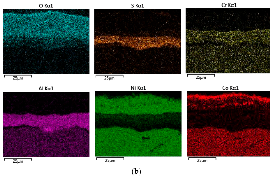
Figure 7. Cross-section of Rene/N5 sample corrosion layers after 300 h LTHC at 700 °C. (a) Secondary electron (SE) image showing two primary layers and internal carbides. (b) Elemental rasters for O, S, Cr, Al, Ni, Co showing inner Cr, Al, S bands and outer Ni, Co bands.
