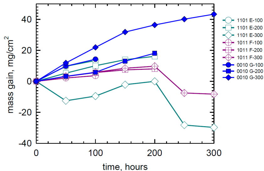
Figure 4. Weight change behavior of duplicate high-Mo LDS SXSA samples in LTHC re-coat furnace tests at 700^\circ\text{C} showing large gains or large losses for specific alloys. See Table 1 for alloy coding. (80\text{Na}-20\text{K})_2\text{SO}_4 sulfate salt spray, 0.5 \text{ mg/cm}^2 every 50 h, 25 h cycles. \text{pSO}_2 = 300 \text{ ppm} in air.
